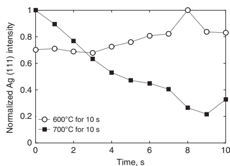
Figure 4 | In situ measurement of Ag diffraction during isothermal heating. Ag(111) diffraction intensity as function of time during heating of Ag/frit (5 wt.% Ag) in air suggests Ag dissolution into the frit at 700 °C, but not at 600 °C.
