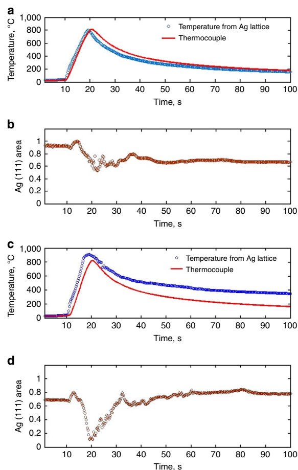
Figure 5 | Temperature profiles and Ag(111) diffraction measured from Ag/frit/ \text{SiN}_x /Si during firing ( 100 \text{ °C s}^{-1} ) and cooling in air and \text{N}_2 . (a,c) shows the temperature measured by thermocouple (red lines) versus calculated based on the Ag peak position (blue lines), and (b,d) shows the Ag diffraction intensity dependence on time. (a,b) corresponds to firing in air, while (c,d) is in \text{N}_2 .
