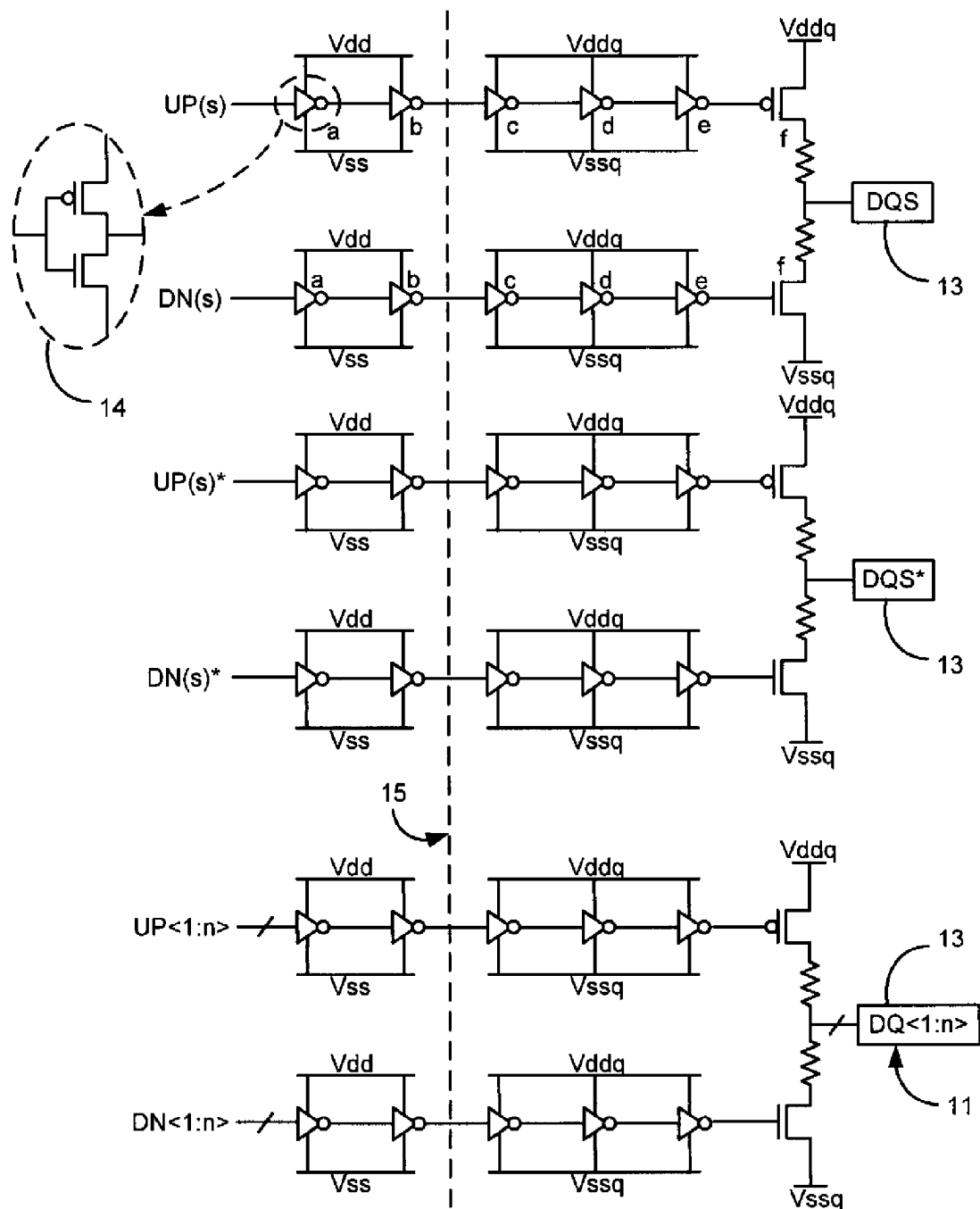
Figure 2 (prior art)
