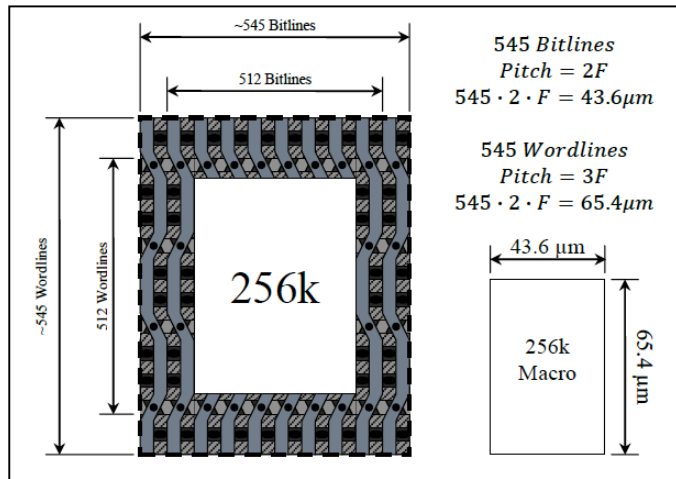
Figure 1. Creation of a 256 kb array
