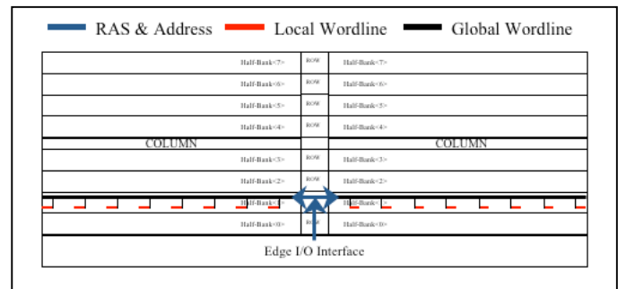
Figure 4. Half-Bank access scheme
