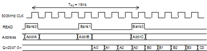
Figure 5. Interleaved Bank Operation
