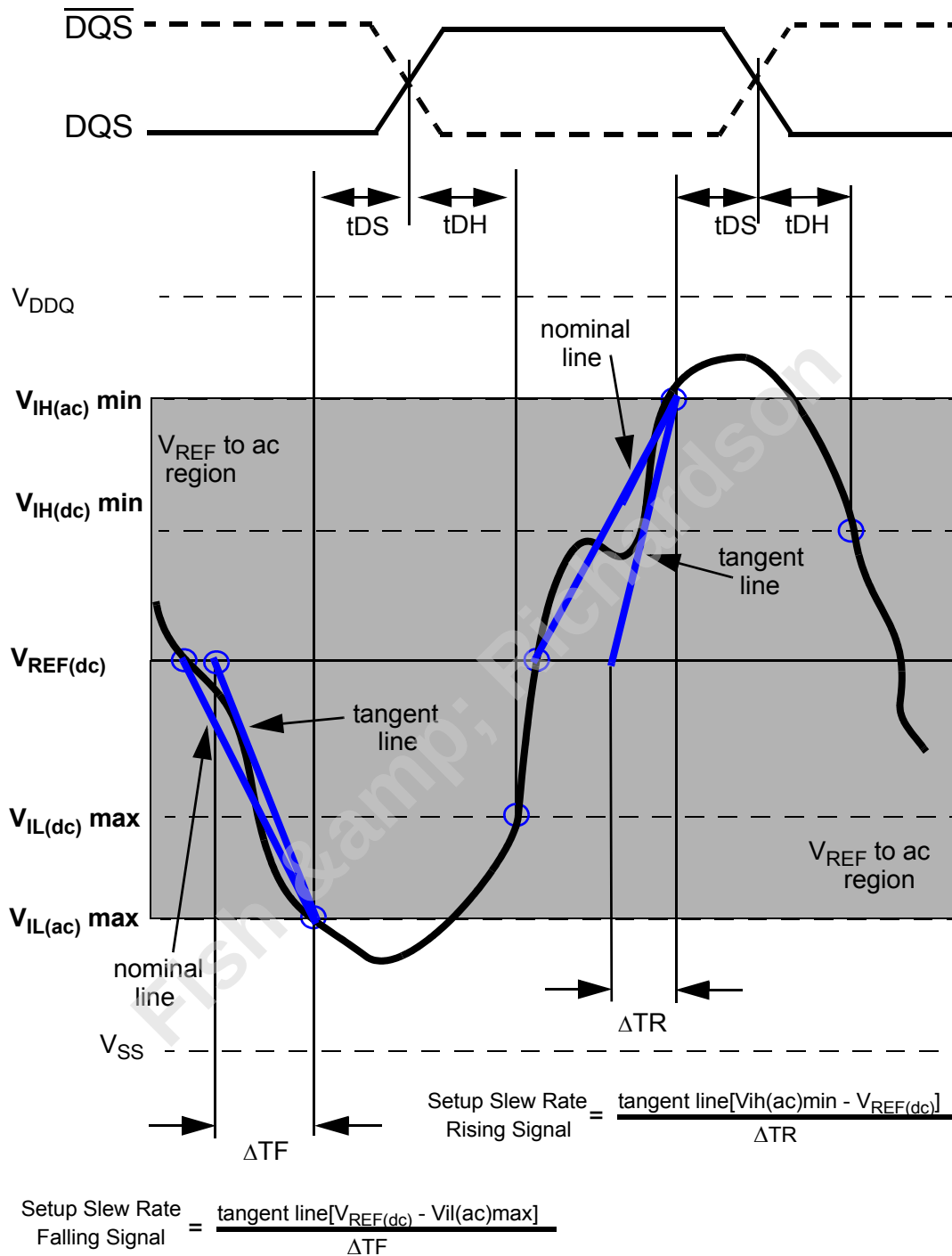
Figure 87 — Illustration of tangent line for tDS (differential DQS, \overline{DQS} )
