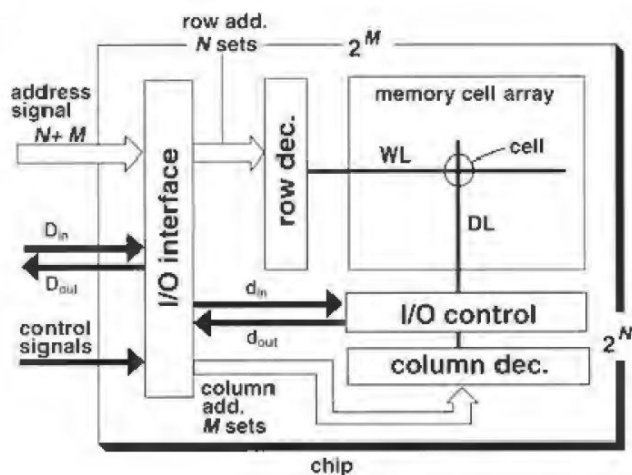
Fig. 1.4. The memory chip configuration
