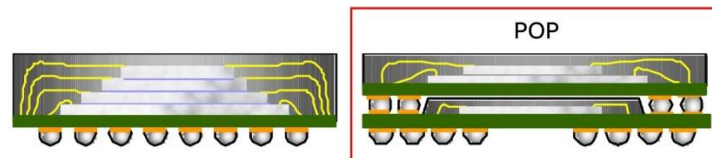
Figure 1: Structure of SCSP and PoP
