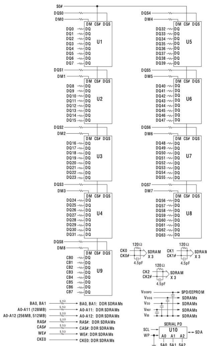
Figure 3: Functional Block Diagram
