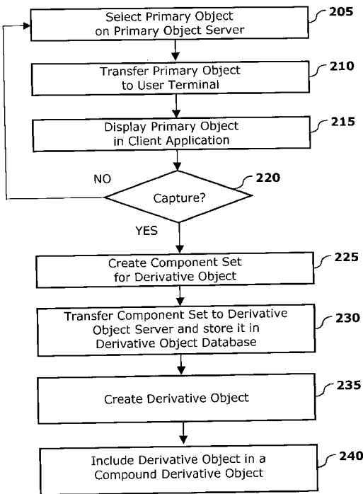
CREATE DERIVATIVE OBJECT (DO) BY CAPTURING COMPONENTS OF PRIMARY OBJECT
