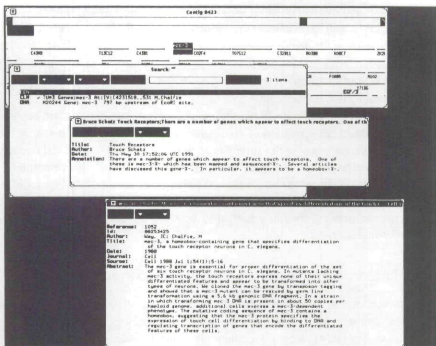
Figure 5. Annotation
