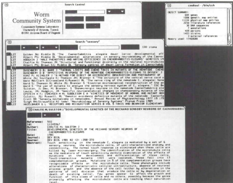
Figure 2. Search
