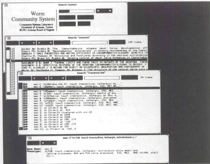
Figure 3. Navigation
