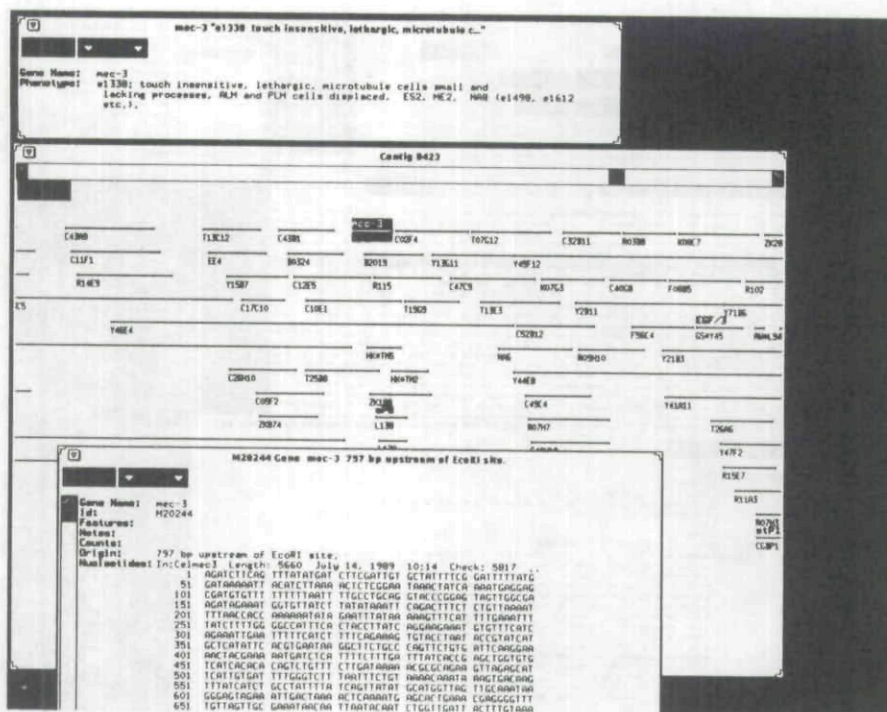
Figure 4. Data Displays
