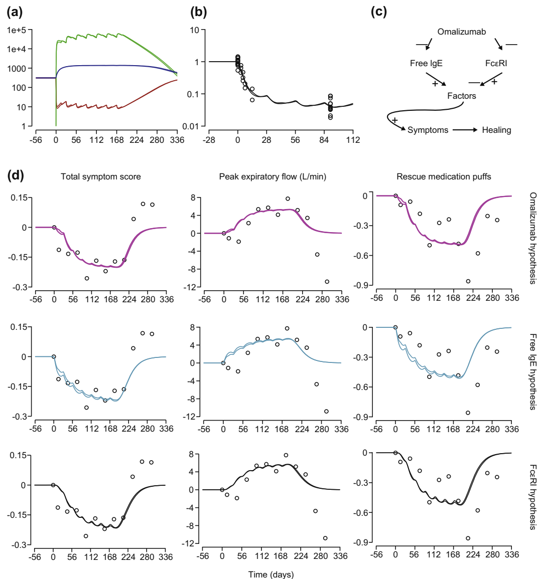
Fig. 7. Omalizumab–IgE model with basophil Fc \epsilon RI and asthma symptoms. (a) simulation of the geometric mean serum concentrations of omalizumab (upper, green), total IgE (middle, blue) and free IgE (lower, red) from 1000 patients 40–150 kg bodyweight, 30–700 IU/mL baseline IgE using the omalizumab dosing table. (b) Basophil Fc \epsilon RI data from MacGlashan et al. (1997) was digitized and fitted with a time-delay indirect response function driven by omalizumab concentrations. (d) Symbols are placebo-corrected changes in asthma symptoms from Slavin et al. (2009), shown together with PK–PD curves representing three causal hypotheses. All three were indirect response functions: pink had omalizumab driving symptom change, cyan free IgE, black omalizumab driving basophil Fc \epsilon RI, which drove symptom change. The simulations were for either the original dosing table or the revision with doses up to 600 mg q4w. To illustrate better any possible differences, the symptom simulations were for the 6 cells covering 40–70 kg bodyweight and 300–500 IU/mL baseline IgE, originally licensed for 225 or 300 mg q2w, now revised to 450 and 600 mg q4w. Within each panel the q4w dosing is that with the slightly larger peak-to-trough variation.
