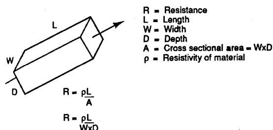
Figure 2.5 Resistance of rectangular bar.
