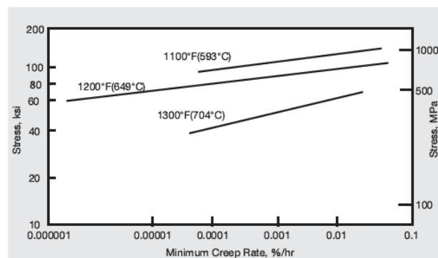
Figure 7. Creep strength of hot-rolled bar 0.625-in. (15.9 mm) diameter (1800°F/982°C)/1 hr, W.Q. and aged 1325°F(718°C)/8 hr, F.C. to 1150°F(621°C), hold at 1150°F(621°C) for total aging time of 18 hr).
