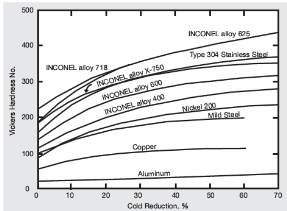
Figure 16. Effect of cold work on hardness.
