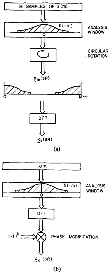
Fig. 1. (a) Generation of the short-time signal x_m(sR) by windowing and circular shifting by M/2 samples. (b) An equivalent method based on a phase modification of the DFT.
