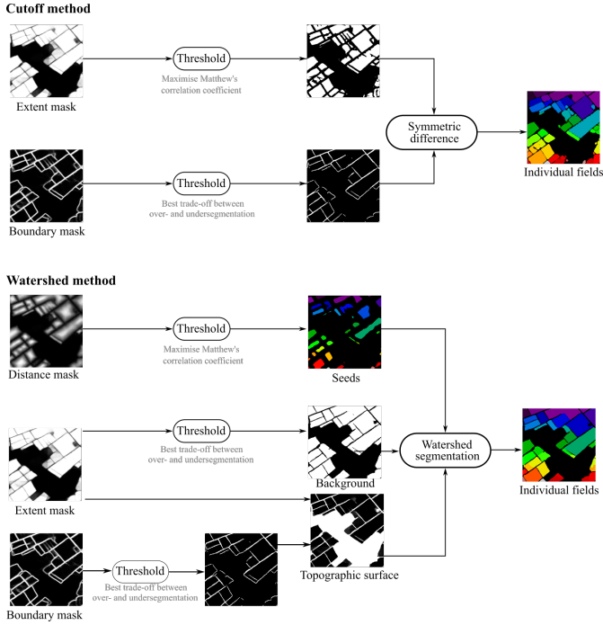
Figure 3: Post-processing methods to generate closed boundaries and extract individual fields. The cutoff method generates individual fields by thresholding and combining the boundary mask and the extent mask. The watershed method extracts fields by all segmentation masks in a watershed algorithm. Seeds for the watershed algorithm are extracted from the distance mask.
