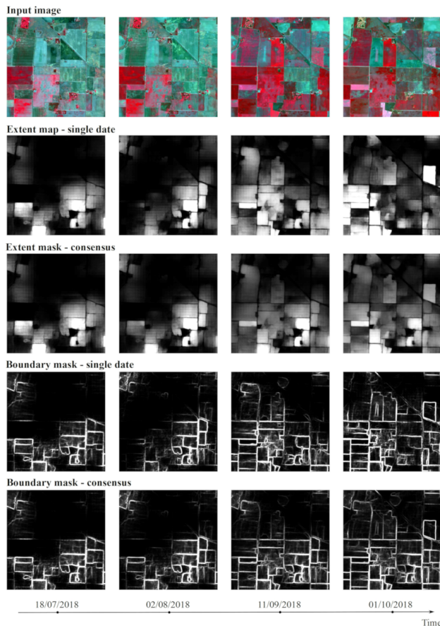
Figure 10: Building consensus for an image subset in Australia. Single-date masks fail to capture all fields and all boundaries but missed patterns can be detected at later in the season. By averaging multiple predictions, the consensus approach is a computationally-cheap option to safeguard against loss of accuracy.
