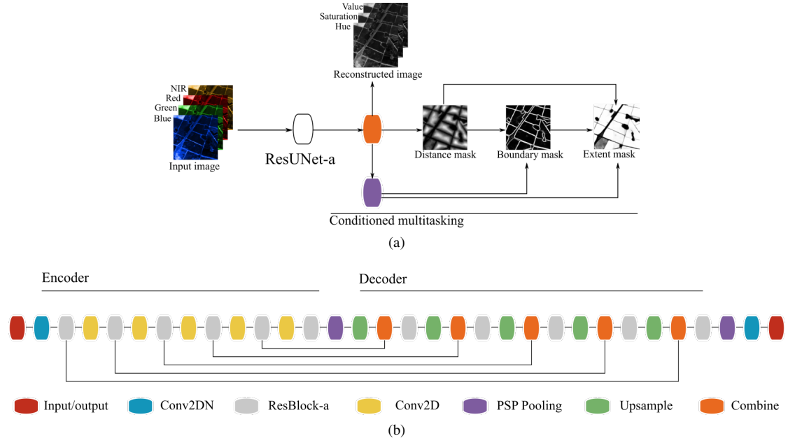
Figure 1: Field boundary extraction formulated as multiple semantic segmentation tasks. (a) Overview of the ResUNet-a's graph for multitasked inference. The distance mask is first generated from the feature map, then is combined to the feature map to predict the boundary mask. Both masks are used to predict the extent mask. An independent branch reconstructs the input image. (b) Architecture of ResUNet-a D6
