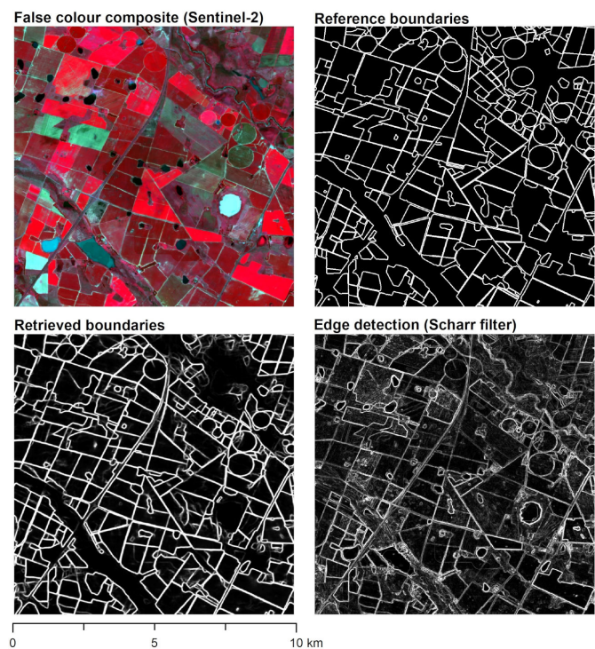
Figure 8: Comparison of the boundaries retrieved by our model against references boundaries and edges detected with a Scharr filter for a 10-km × 10-km region in the test region (27°E 49°, 27°S 30”).
