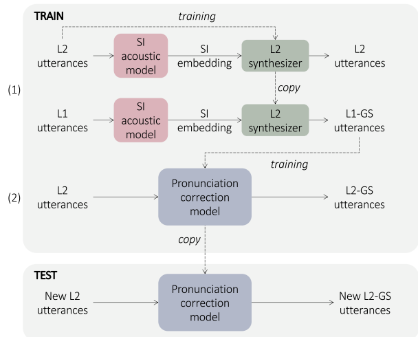
Fig. 1. Overall workflow of the proposed system. L1: native; L2: non-native; GS: golden speaker; SI: speaker independent. The training stage consists of two steps. In step 1, we use a conventional FAC procedure to generate a set of golden-speaker utterances (L1-GS), which serve as targets for step 2. In step 2, we train a pronunciation-correction model that converts L2 utterances into the L1-GS utterances obtained earlier. Once the pronunciation correction model is trained, in the testing stage, a new L2 utterance is processed by the pronunciation-correction model to create its “accent-free” counterpart (L2-GS).
