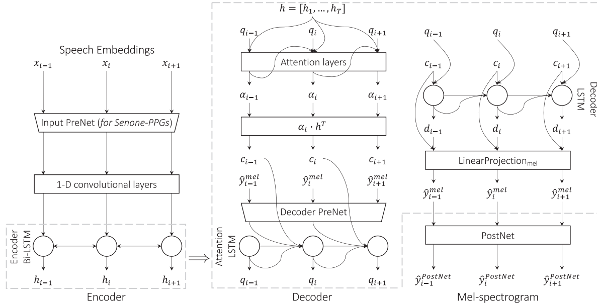
Fig. 3. Speech embedding to Mel-spectrogram synthesizer. The speech embeddings are sequentially processed by an input PreNet (optional, for Senone-PPGs only), convolutional layers, an encoder, a decoder, and a PostNet to generate their corresponding Mel-spectra. We omitted the stop token predictions in the figure for better visualization.
