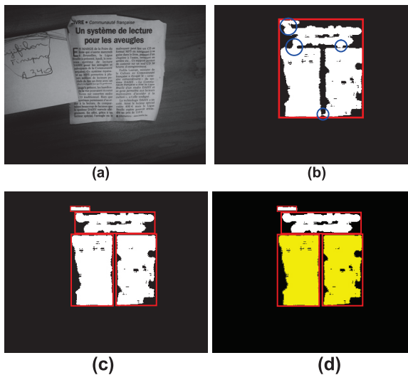
Figure 8. (a) Original image (b) Illustration of text regions to separate (c) Results after iterative columns & paragraphs separation (d) Illustration of detection of columns
