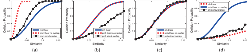
Fig. 4. Simulated collision probability of partition min-hash with overlapping partitions for four cases. ‘mh theor’: Theoretical rate of standard min-hash. ‘pmh theor no overlap’: Theoretical rate of partition min-hash with non-overlapping partitions. ‘pmh simul overlap’: Simulated rate of partition min-hash with overlapping partitions.
