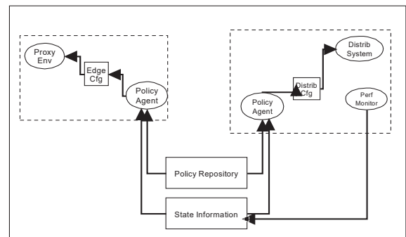
Fig. 3. A policy based Architecture for content distribution networks.
