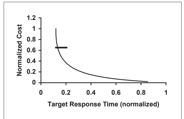
Fig 6 . The cost of supporting a response time SLA with and without dynamic policies. The normal line shows the cost of a dynamic solution. The thick horizontal line shows the constant cost of supporting a response time without dynamic content distribution policies, but the static planning can not support a response time below 0.12. Dynamic distribution policies can offer smaller target response times, as well as reduce cost for larger target response times.
