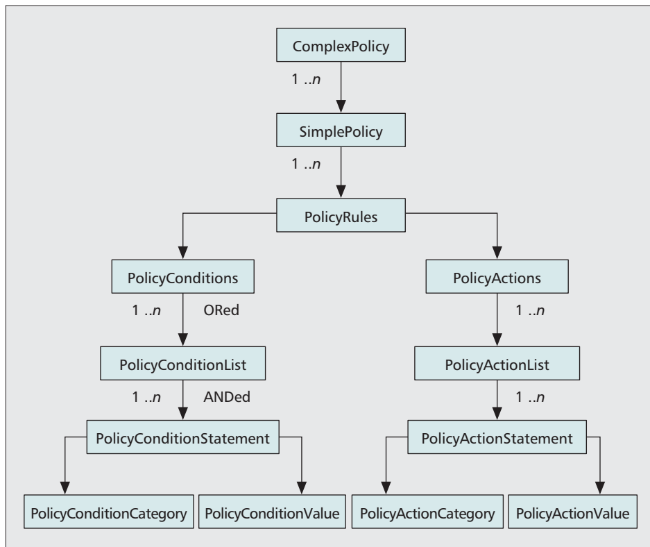
■ Figure 3. A PFDL hierarchy.
