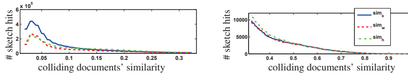
Figure 1: The number of sketch hits as a function of the document similarity for different similarity measures (TrecVid data set). Left: similarities 0 – 0.35, right: high similarities (different scale).
