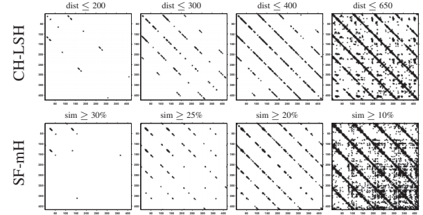
Figure 13: Dependence of the scene repetition retrieval in ‘Come Into My World’ on varying thresholds.
