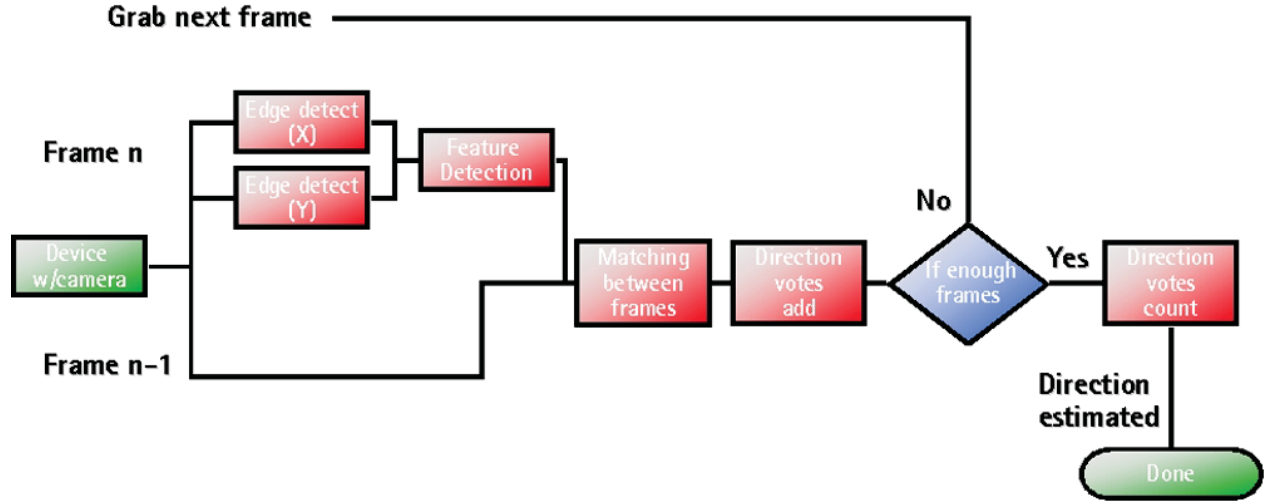
Figure 3: Our tracker uses the current and previous frame captured by the camera for tracking. Corner like features are detected in the new frame which are matched with the features found in the prior frame so that the prior frame does not have to be reprocessed for features. Direction estimates are accumulated for a number of frames before a movement direction estimate is made.
