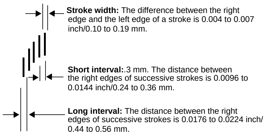
Figure 4-8. CMC7 stroke and interval dimensions
