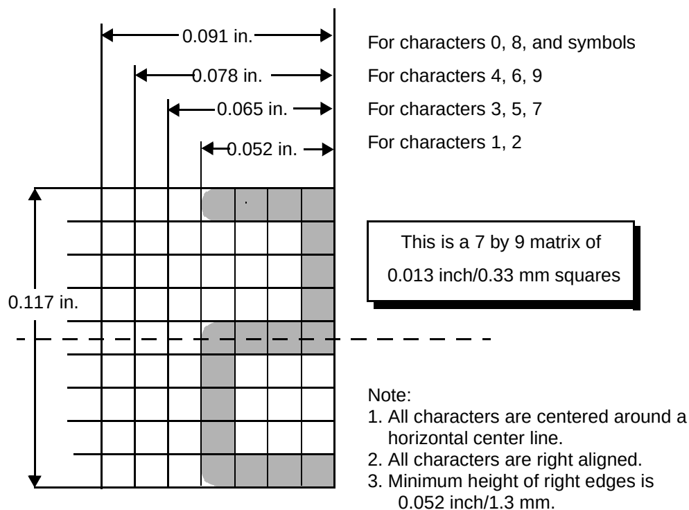
Figure 4-3. E13B character matrix design
