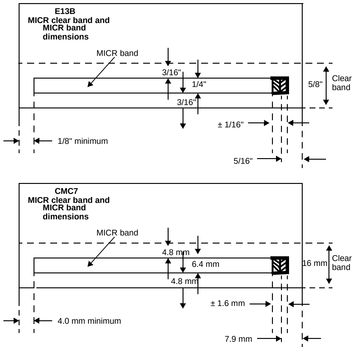
Figure 4-2. MICR clear band dimensions
