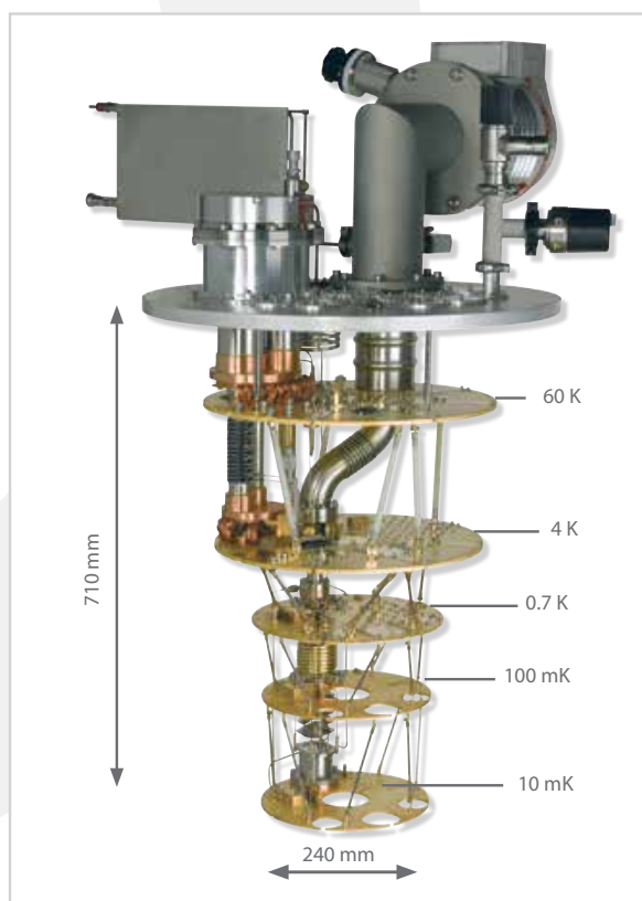
Internal assembly of a Cryofree dilution refrigerator
