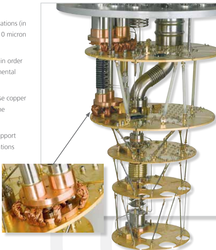
Internal assembly of a Cryofree dilution refrigerator
