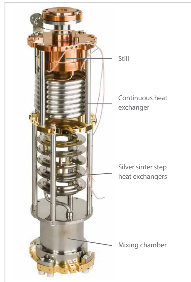
Dilution unit for operations below 10 mK
