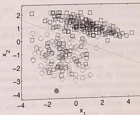
Figure 4. CE classifier for synthetic problem (0.333% SVs).
