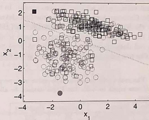
Figure 3. One-norm SVM classifier for synthetic problem (0.667% SVs).
