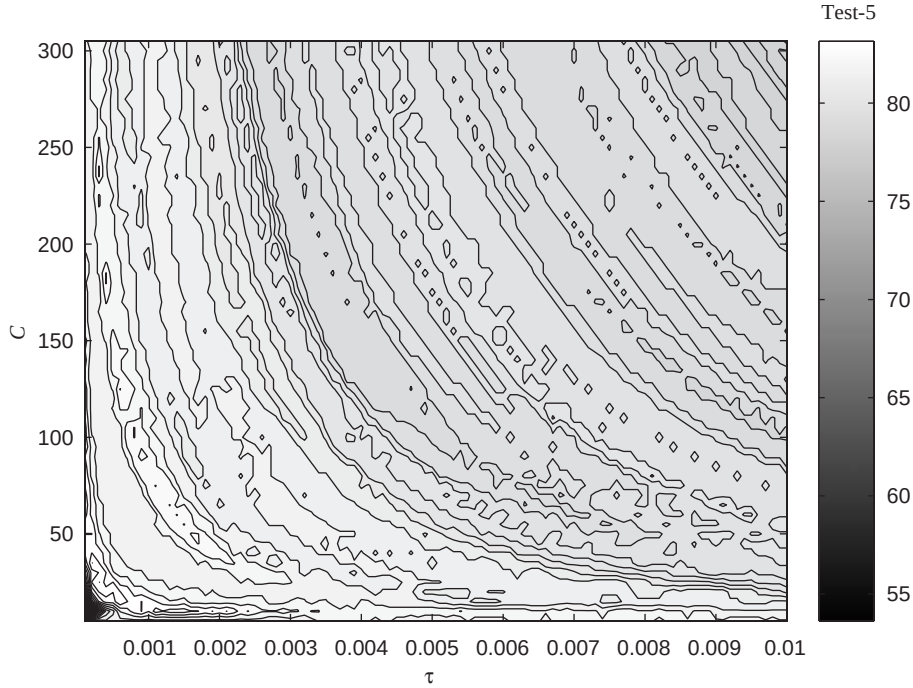
Fig. 1. Score function (average classification rates on the five test sets, Test-5, in percent) for the Heart dataset using K_{\tau I} with different combinations of C and \tau .
