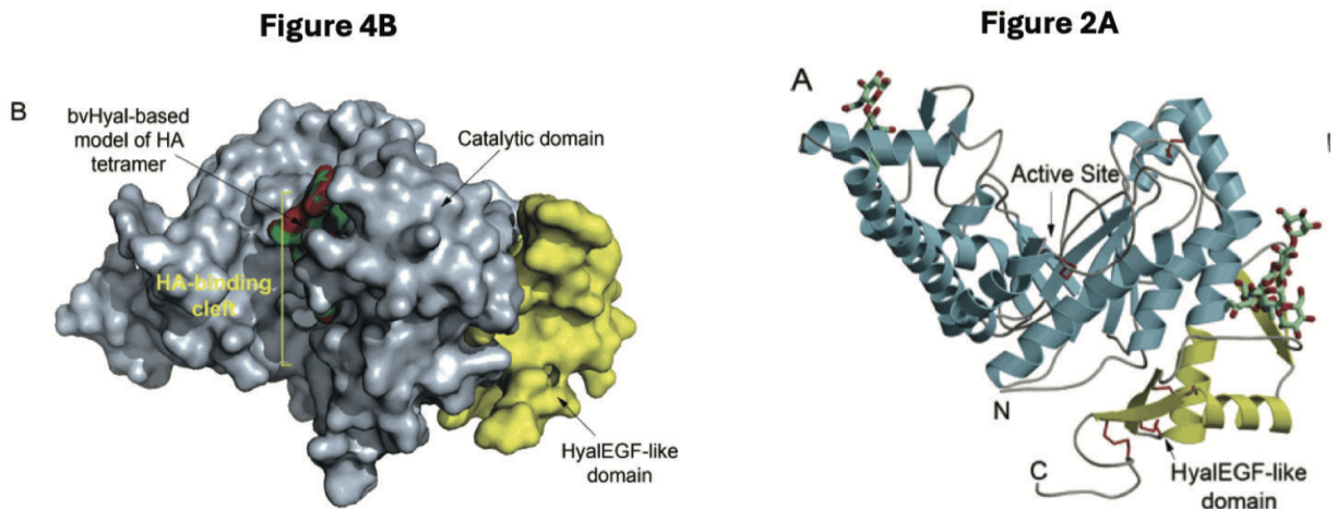
FIGURE 4: (B) Molecular surface of the catalytic domain (light blue) and HyalEGF-like (yellow) domains of hHyal-1, illustrating the separation between the HyalEGF-like domain and the active site. A docked tetrasaccharide, inferred from the structure of bvHyal, is shown as a space filling model.
