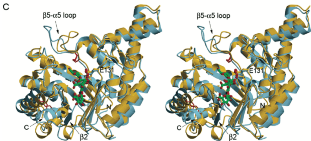
FIGURE 2: Structure of hHyal-1. (C) Stereoscopic representation of the catalytic domain (colored light blue) superimposed on the structures bvHyal in complex with (GlcUA-GlcNAc) 2 (colored gold; (22), PDB entry code 1FCV). The tetrasaccharide is colored with an atomic color scheme: green, carbon; red, oxygen; blue, nitrogen.
