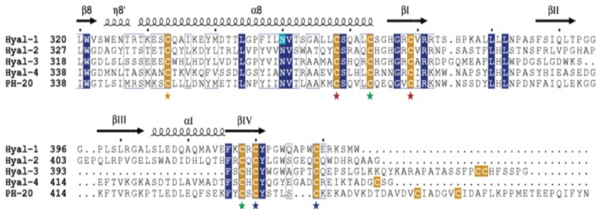
FIGURE 3: Structure-based sequence alignment of human hyaluronidases. Invariant residues are shown in blue except for three key catalytic residues that are colored red. Cysteine residues are colored yellow. The hHyal-1 N-glycosylated asparagines residues are colored turquoise. Residues exhibiting conservative replacements are blocked in blue. Pairs of cysteine residues that form disulfide bonds are indicated by stars with matching colors. Secondary structure units are labeled as in Figure 2B.
