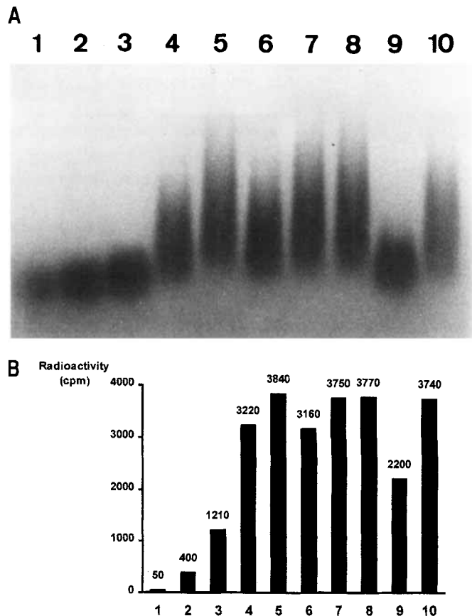
Fig. 4. Assays for hyaluronidase activity. (A) Hyaluronan was incubated for 2 h with 20 \mu l Triton X-100 extracts, which corresponds to about 4 \times 10^5 cells expressing mutant PH-20 proteins. The remaining hyaluronan was fractionated by agarose gel electrophoresis and gels were stained with Stains-All (see Experimental Procedures section). The assay with [ ^{14} C]hyaluronan is shown in B. Triton X-100 extracts prepared from cells infected with recombinant vaccinia virus were incubated with radioactive hyaluronan for 2 h. After paper chromatography, radioactivity remaining at the origin, expressed as cpm, was measured (number above the bars). For comparison, decreasing amounts of wild-type PH-20 hyaluronidase were assayed under the same conditions. Lanes 1–4, aliquots of 1/5, 1/10, 1/20 and 1/100 the amount of extract from cells expressing wild-type PH-20 hyaluronidase; lane 5, blank without enzyme; lane 6, mutant [Gly176]PH-20; lane 7, mutant [Thr252]PH-20; lane 8, [Gln113]PH-20; lane 9 [Asn111]PH-20; lane 10, [Gln249]PH-20. In three separate experiments, 97.2–98.3% of the counts were recovered at the origin for mutants in lane 7, 8, and 10; 79.3–84.0% in mutant [Gly176]PH-20 (lane 6, five experiments, average 82.1); 51.2–59.2% for mutant [Asn111]PH-20 (lane 9, five experiments, average 54.2).
