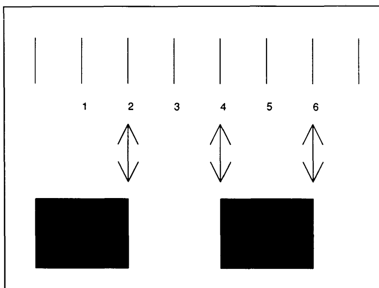
Figure 2. Derivation of the UPC code words. The seven modules (top line) have six boundaries (second line). A partition of the modules into two bars and two spaces requires three internal boundaries that can be placed in each of six locations.
