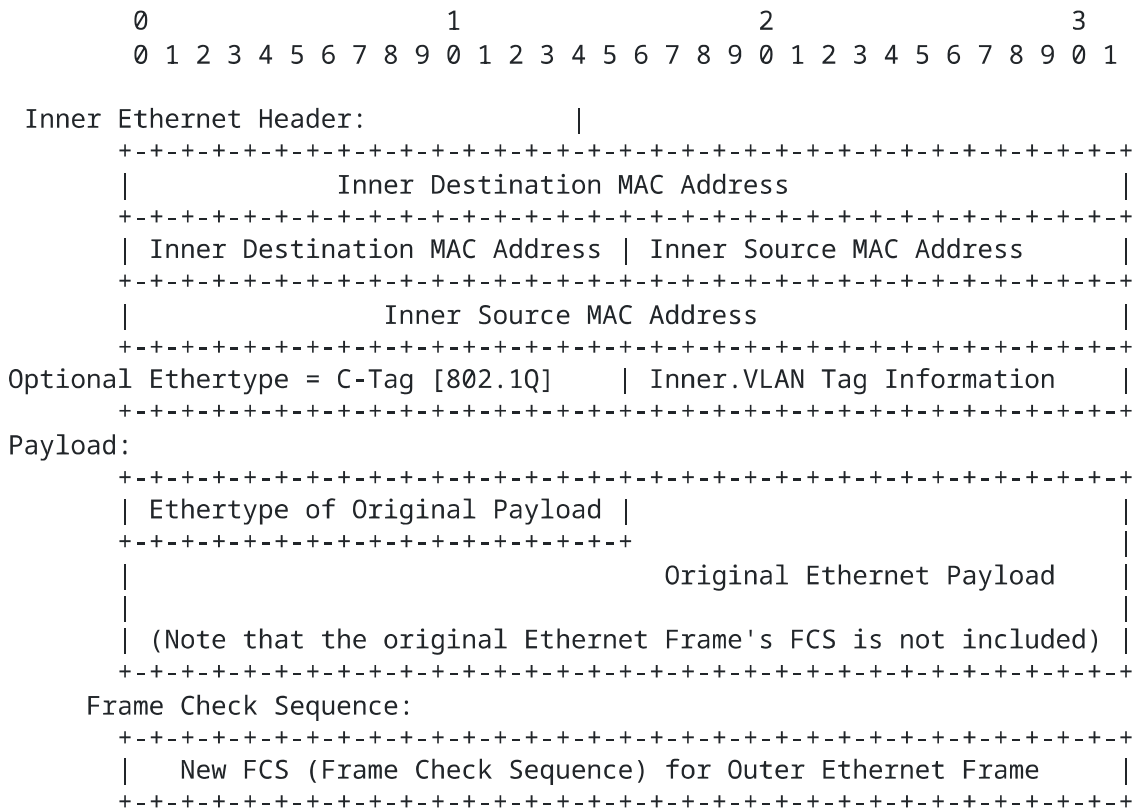
Figure 1 VXLAN Frame Format
