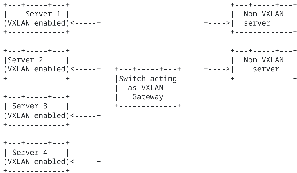
Figure 3 VXLAN Deployment - VXLAN Gateway
