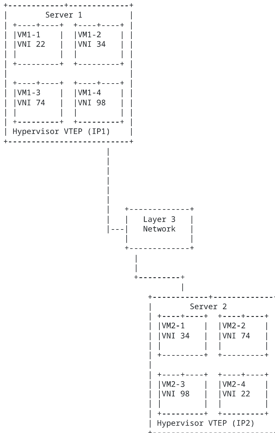
Figure 2 VXLAN Deployment - VTEPs across a Layer 3 Network
