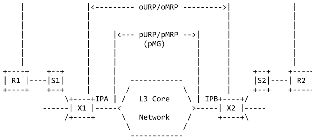
Figure 3. OTV Control Plane Hierarchy
