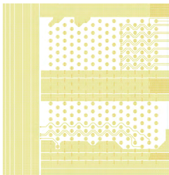
Figure 7.16: Horizontal power distribution on copper layer together with control signals.
