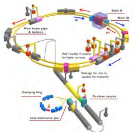
Figure 3.14: Schematic view of SuperKEKB accelerator. [26]
