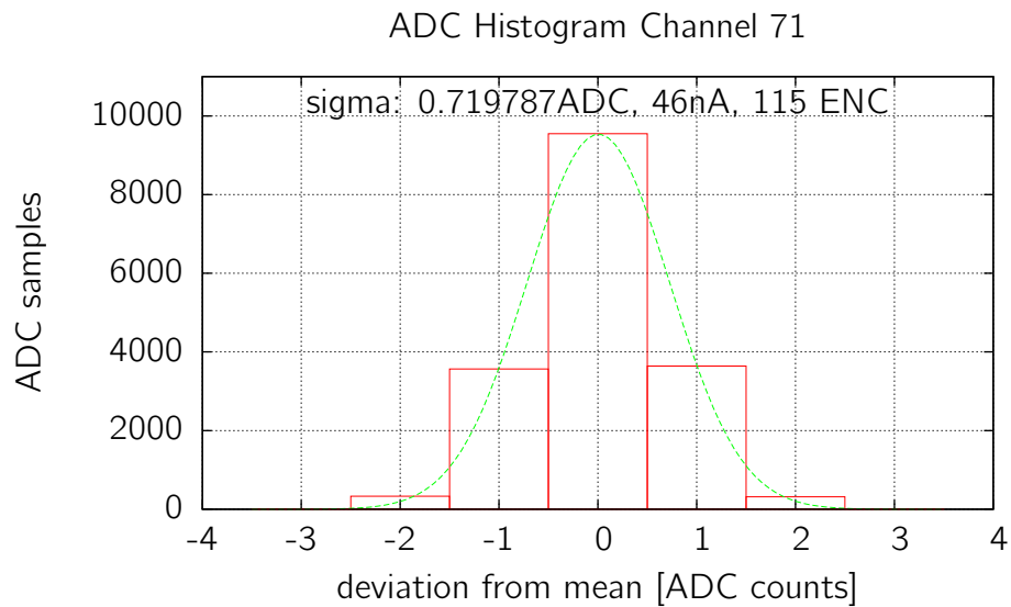
Figure 4.8: DCD2 ADC histogram showing deviation from mean of several ADC samples running at 48MHz. Sigma of 0.7ADC \leftrightarrow 46nA \leftrightarrow 115ENC with g_q = 400pA/e^-
