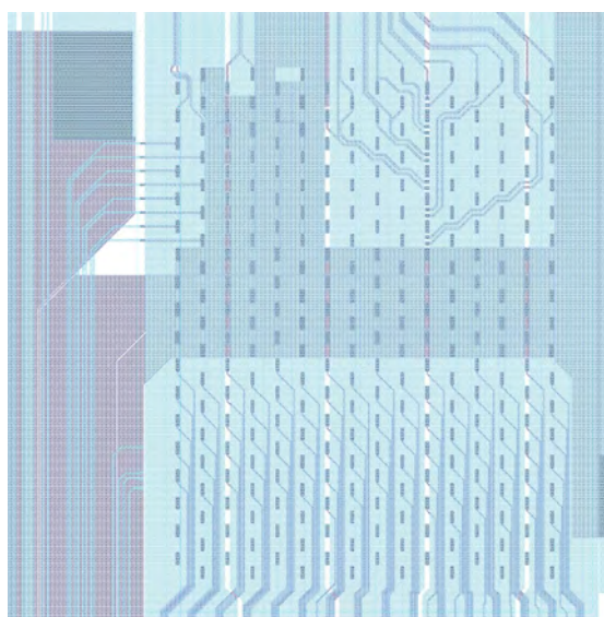
Figure 7.15: Data and control signals and part of the power routed on all layer.
