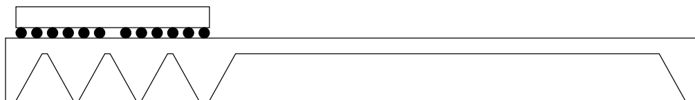
Figure 3.6: Schematic side view of a thin module with a hole pattern in the support frame and a steering chip attached by bump bonding.
