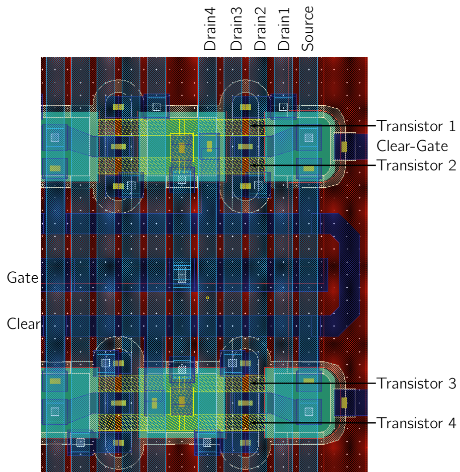
Figure 7.5: Layout of 8 DEPFET transistors with 4-fold read-out. The shown area covers roughly 2x4 pixels which are read out by one gate/clear row and 8 drain lines.
