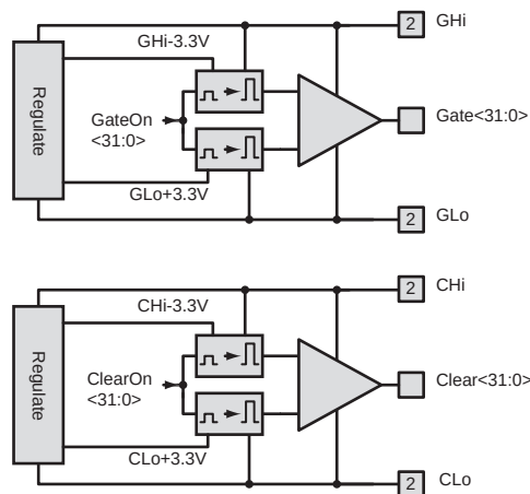
Figure 5.17: Block diagram of the Switcher-B output driver[42]
