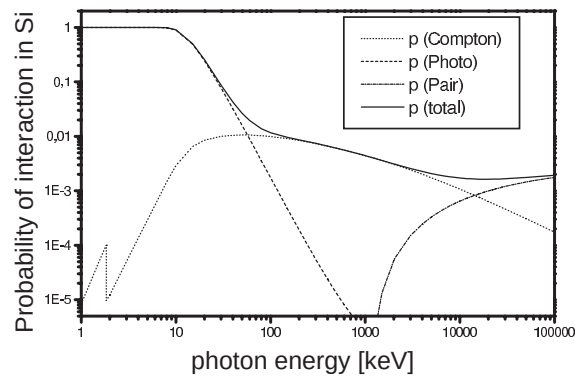
Figure 2.3: Probability of energy loss of a photon in silicon. [6]
