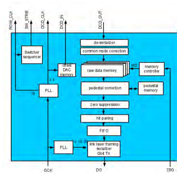
Figure 3.22: Block diagram of the DHP data processing chip. [36]
