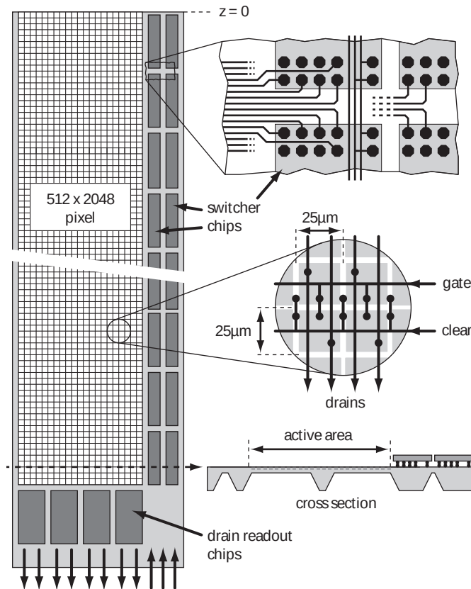
Figure 3.10: ILC half module drawing with cross section of the thinning, double row organization and chip location. [22]
