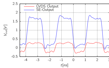
Figure 4.14: Measured DCD-RO LVDS and single ended outputs running at 400MHz.
