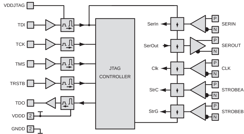
Figure 5.16: Block diagram of the Switcher-B JTAG controller and boundary scan chain. [42]
