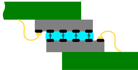
Figure 6.37: CCPD1 Detector assembly principle with PCBs (green) and flip-chip bonded chips (gray) with glue (cyan) to assist capacitive coupling. Both chips are wire bonded.
