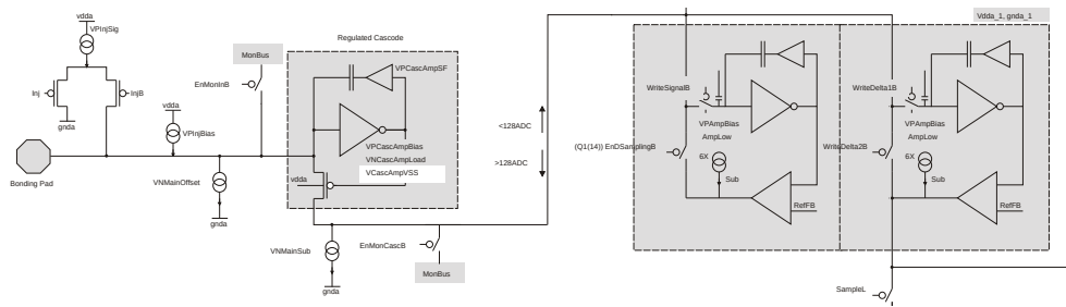
Figure 4.2: Block diagram of input, regulated cascode and current memory cells for double sampling of DCD2. [37]
