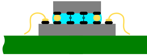
Figure 6.40: CCPD2 Detector assembly principle with the read-out chip (top) flip-chip bonded to the detector (bottom) with glue (cyan) to assist capacitive coupling. Only the detector is wire bonded. Power is supplied to the read-out chip via bump bonds, while the signals are still transmitted capacitively.
