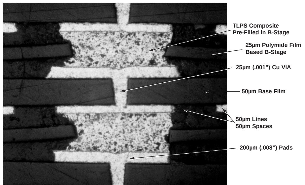
Figure 11-36. Ormet® TLPS Conductive Composite Between 200µm Pads
