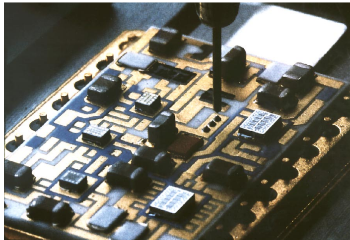
Figure 11-39. Close-Up of a Thick Film Substrate
