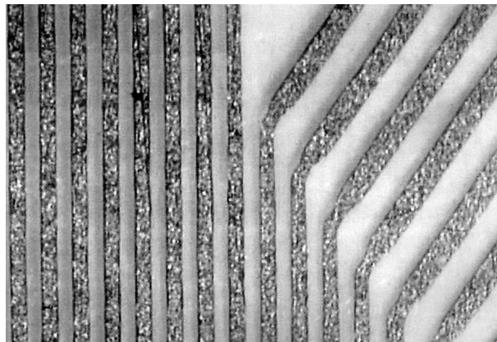
Figure 11-31. 50 Micron Traces on Flex
