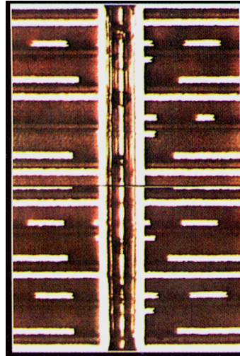
0.15mm Hole Diameter 1.2mm Thick Panel
