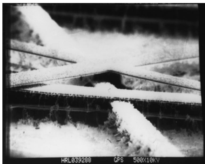
Figure 11-54. Multilayer Thin-Film Interconnect with the BCB Polymer Removed Using Plasma Etching
