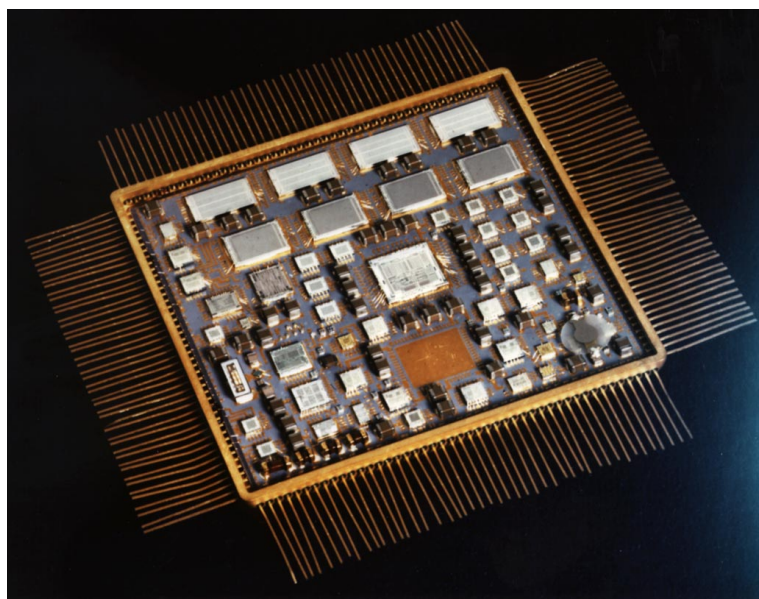
Figure 11-37. 68020 Computer Module on Thick Film Substrate
