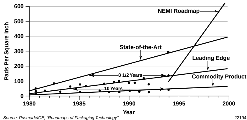
Figure 11-2. Surface Pad Density Over Time
