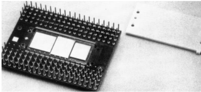
Figure 11-57. Silicon Substrate Packaging
