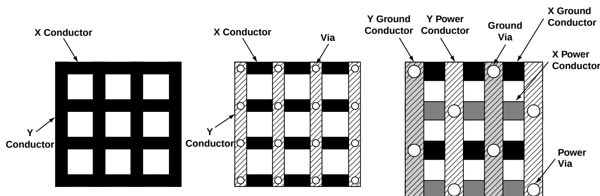
Figure 11-65. IMPS: Intermeshed Power System
