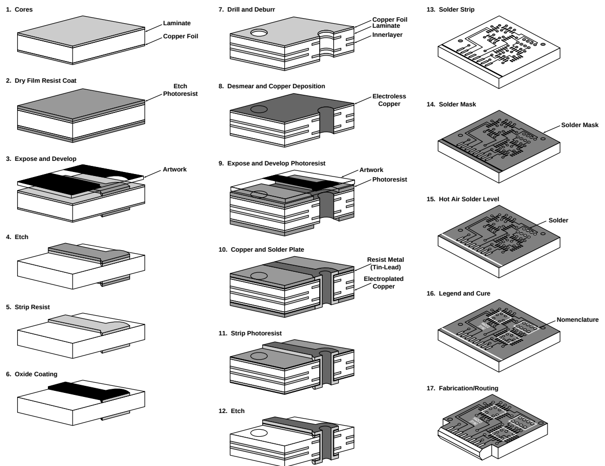
Figure 11-3. How to Build a Circuit Board
