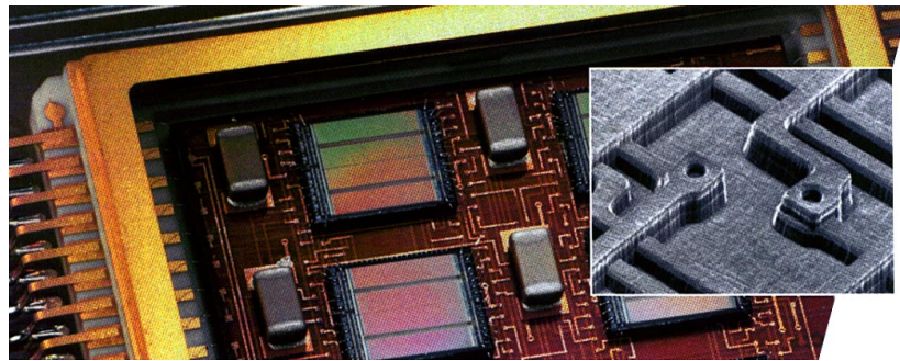
Laser \mu Vias on an MCM
