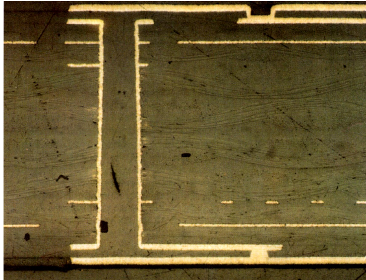
Figure 11-27. Cross Section of a Plasma-Produced Eight-Layer Micro Via Board Showing Blind Vias and a Buried Via Core
