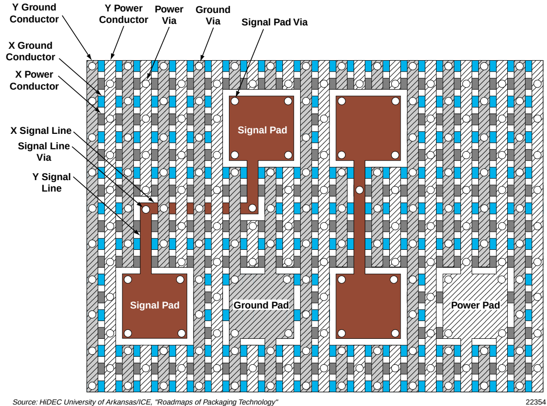
Figure 11-67. IMPS with Routing of Pads
