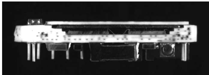
Figure 11-43. Cross Section of Cofired Ceramic Hybrid Pacemaker
