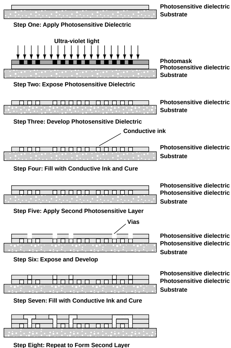
Figure 11-34. Multilayer Fine-Line Printed Circuitry Using Toranaga's Process
