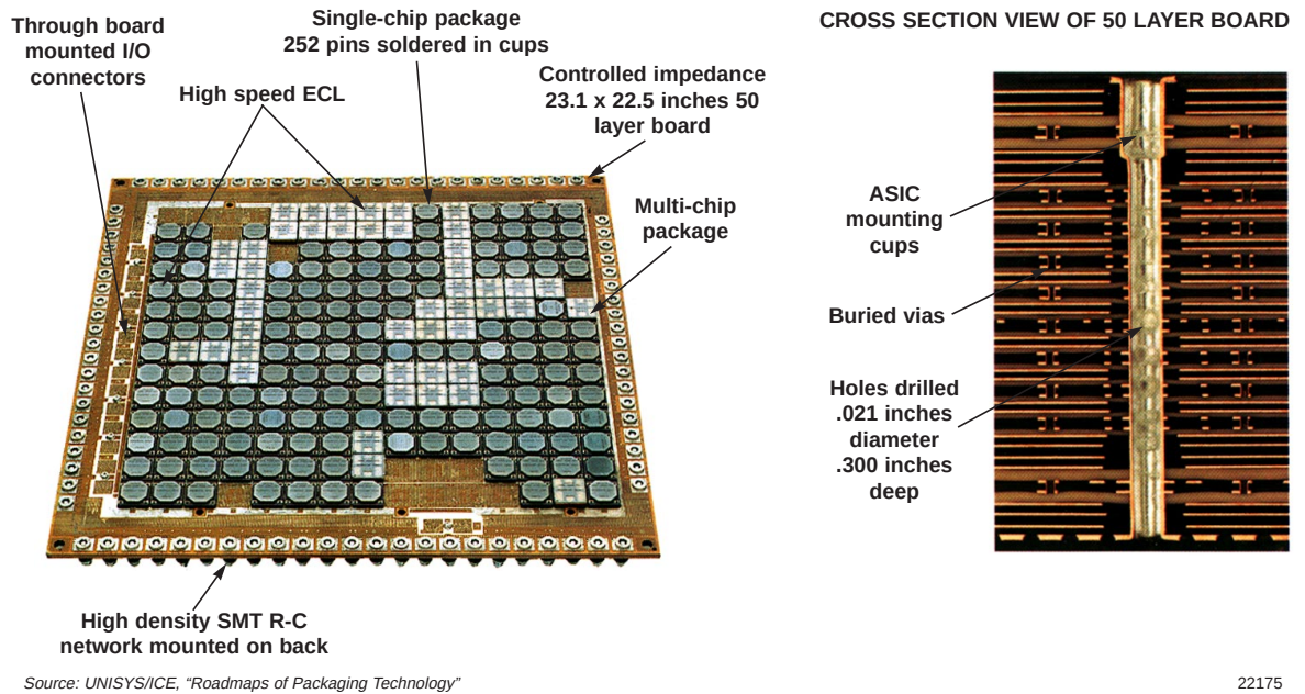
Figure 11-9. 50 Layer Board
