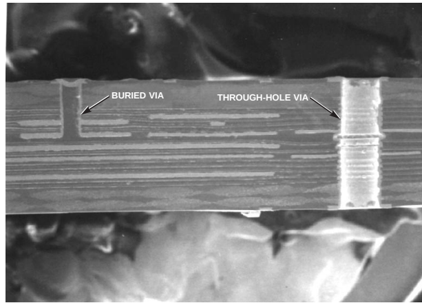
Figure 11-14. Buried Via and Through-Hole Via
