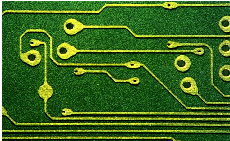
Figure 11-23. Close Up of SLC Substrate with Mechanically Drilled Holes and Photoimaged Micro Vias
