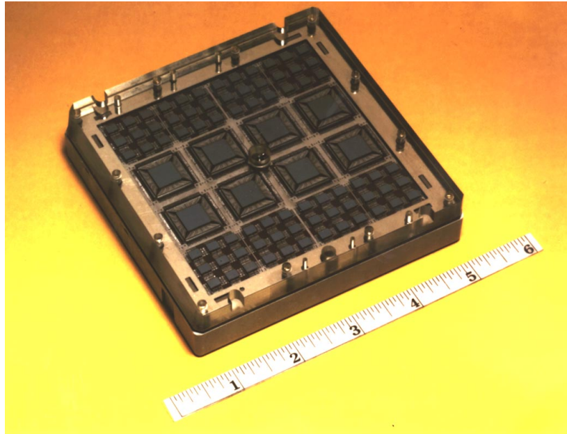
Figure 11-22. 80-Chip Bipolar MCM Using Fine-Line PWB Interconnect Substrate
