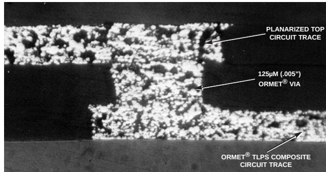
Figure 11-35. Ormet® TLPS Conductive Material in Circuit Traces and Vias
