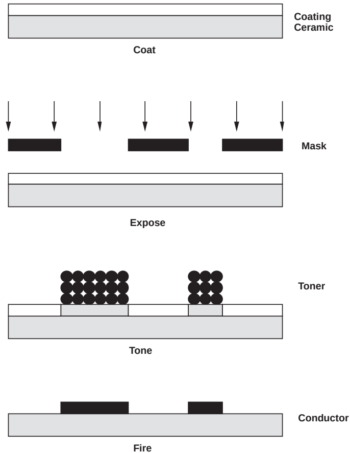
Figure 11-41. PCS Process
