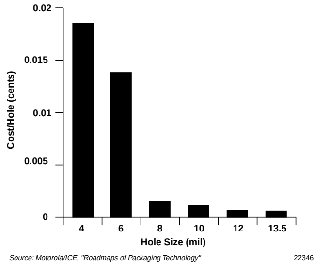
Figure 11-21. Drilling Cost Versus Hole Size
