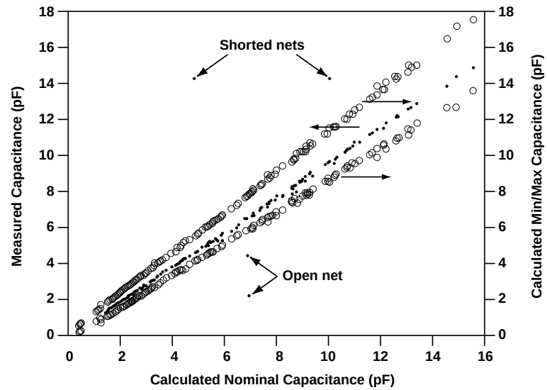
Figure 11-70. Using Capacitance to Identify Opens and Shorts
