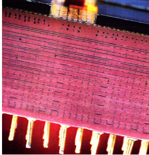
Figure 11-47. Cross Section of 52 Layer Cordierite Substrate with 1 Layer Thin Film-Polyimide on Top
