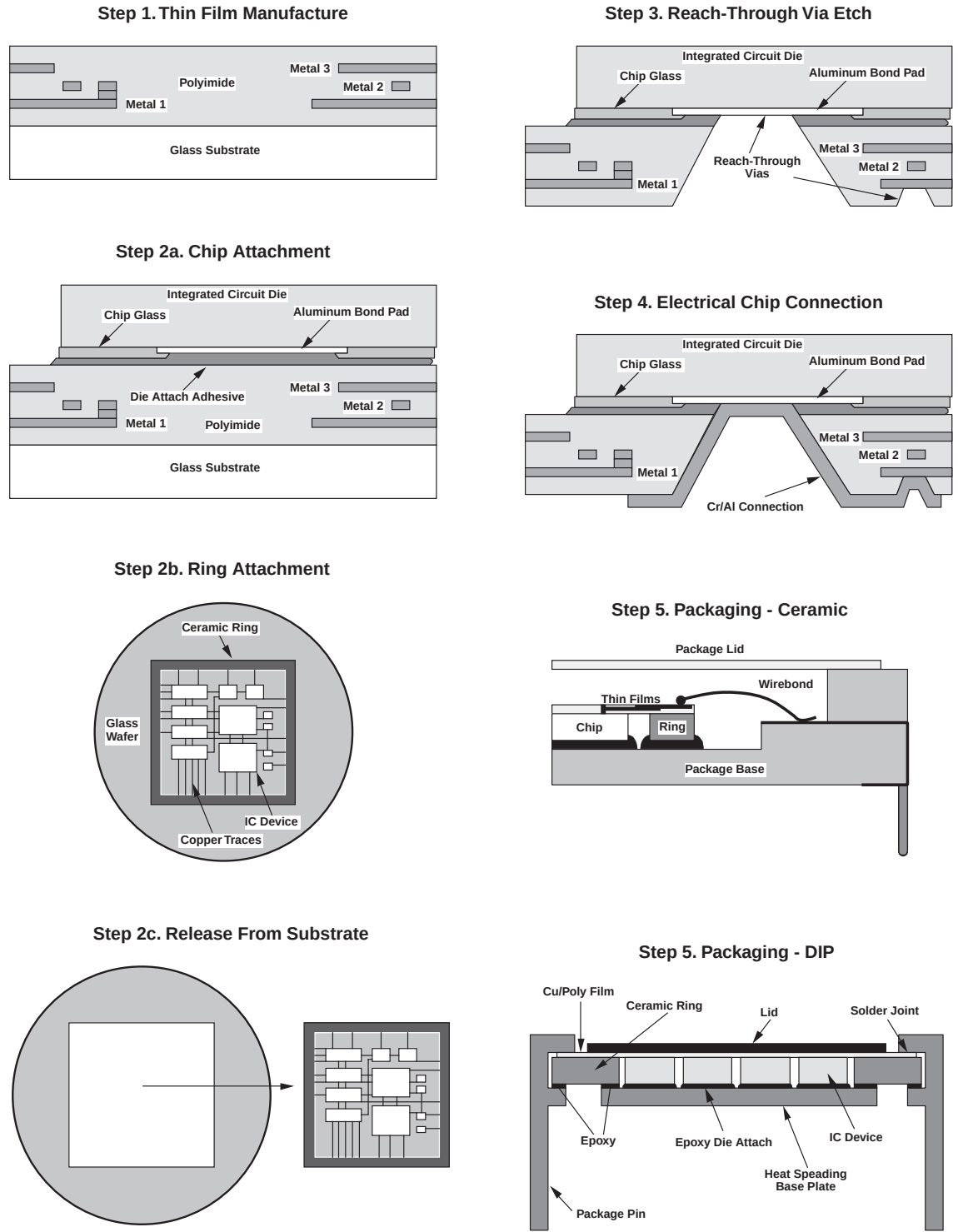
Figure 11-63. Free-Standing, Thin-Film Multilayer Interconnect
