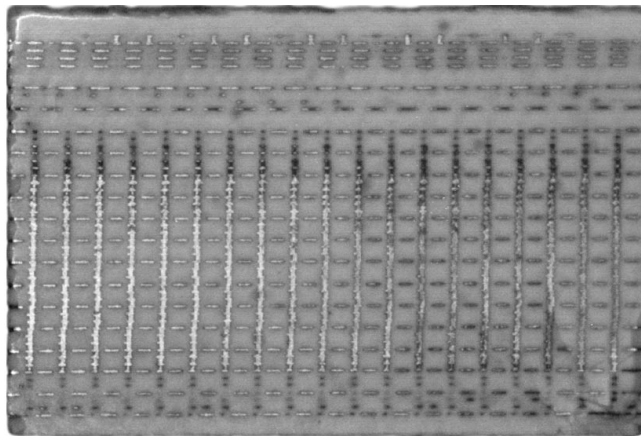
Figure 11-46. Cross Section of 62 Layer LTCC Substrate Used in the Fujitsu VP2000 Super Computer
