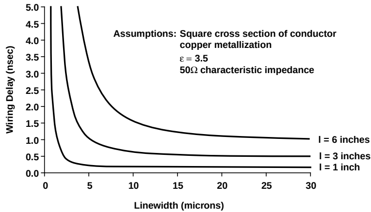
Figure 11-64. Wiring Delay of Thin-Film Interconnects
