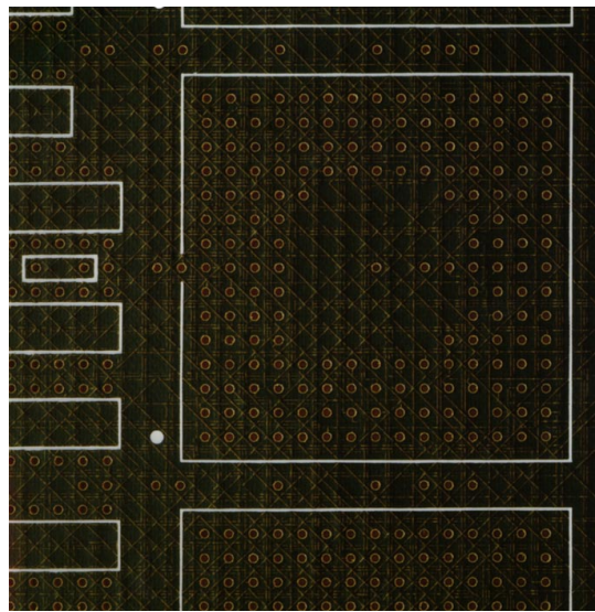
Figure 11-19. Diagonal Wiring Multiwire Boards
