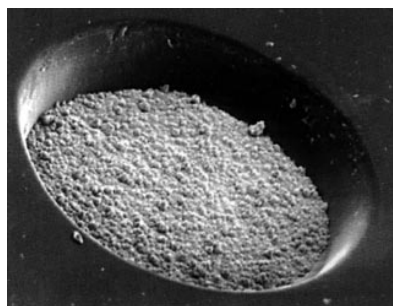
150 \mu m Laser Drilled Blind Via in Polyimide
