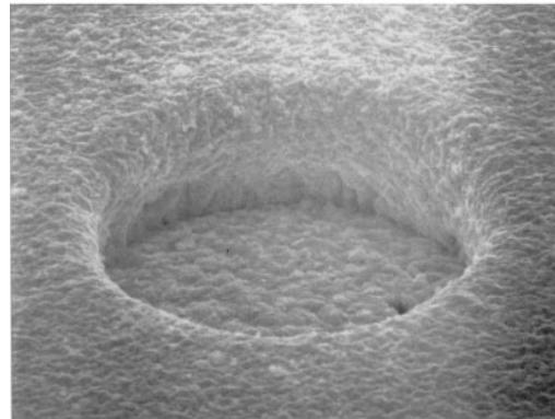
Figure 11-56. 35 \mu Via in Polyimide Before and After Metallization
