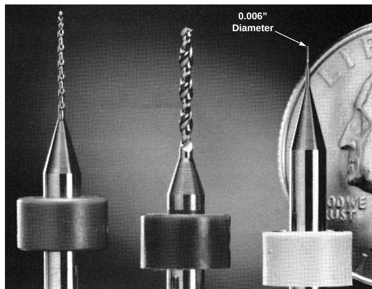
Figure 11-4. Various Drill Bit Diameters
