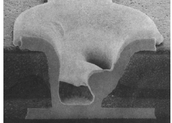
Cross Section of a Lased Via After Metallization
