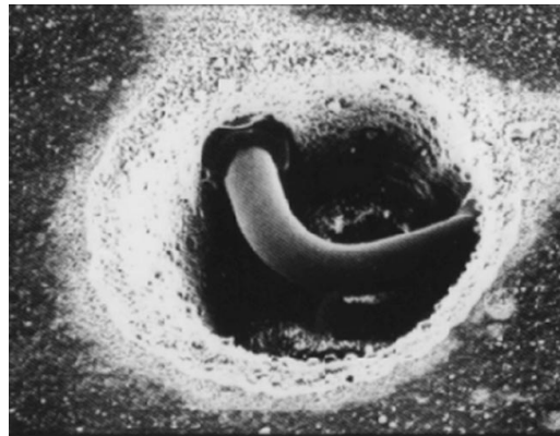
2.5mil Wire Passing Through a Lased Hole
