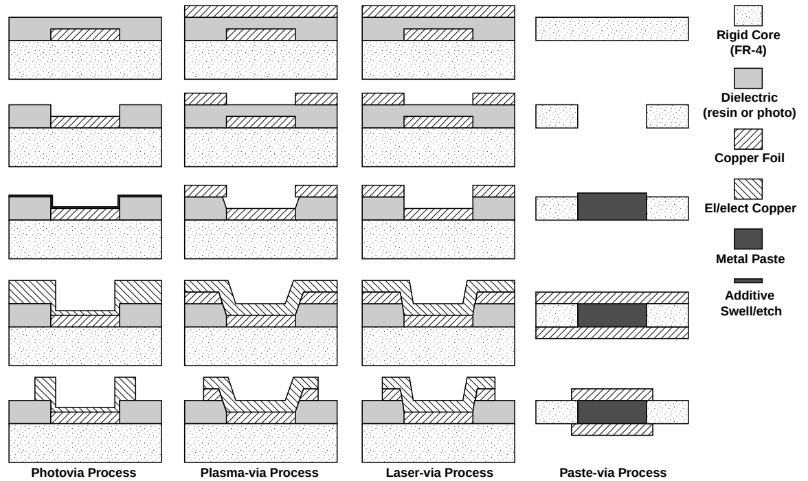
Figure 11-30. \mu Via Process Flow
