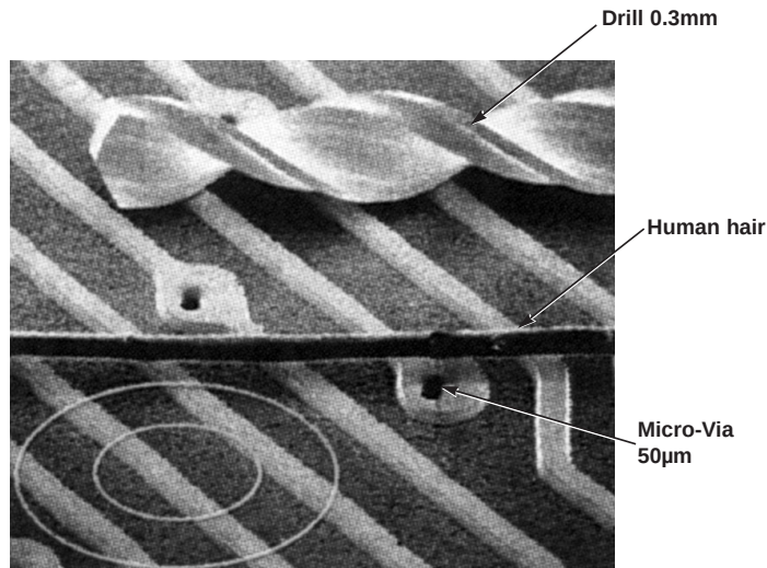
Figure 11-33. Comparison of 50µm Microvia Fabricated by Plasma Etching and 12mil Drill Bit
