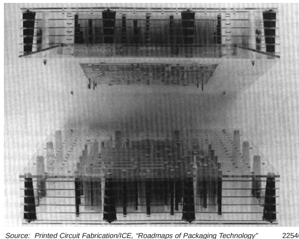
Figure 11-68. A Double-Sided Universal Grid System
