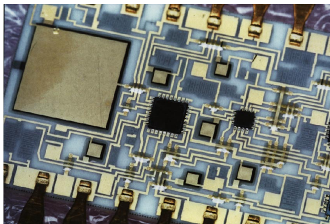
Figure 11-49. AT&T Beam-Lead Hybrid
