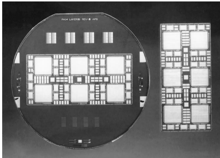
Figure 11-60. 125mm Round Ceramic Substrate and Diced Component
