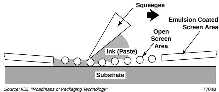
Figure 11-38. Screen Printing Process
