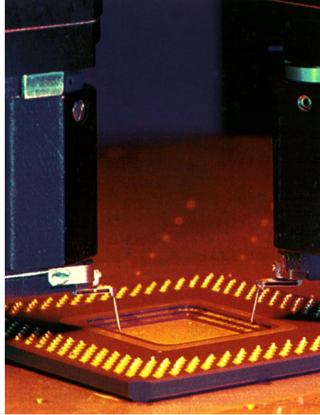
Figure 11-72. Dual Probe Heads for Capacitance and Resistance Testing
