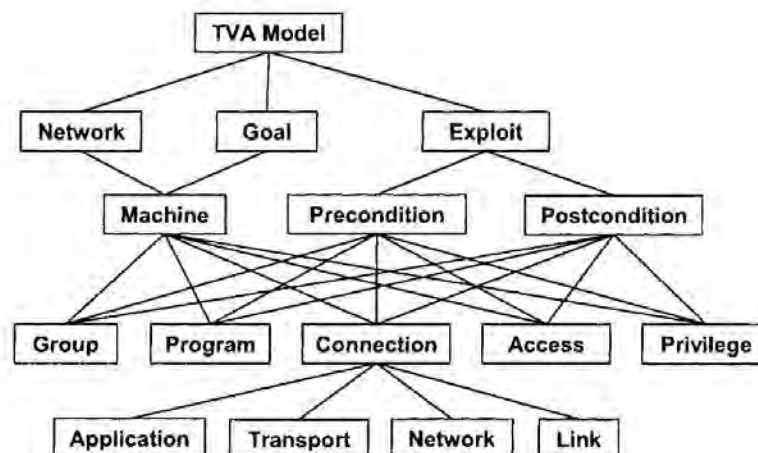
Figure 9-2. TVA Model Structure
