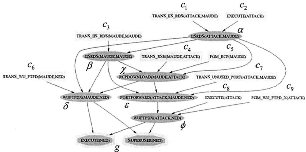
Figure 9-7. Attack Graph with Exploit Preconditions Included
