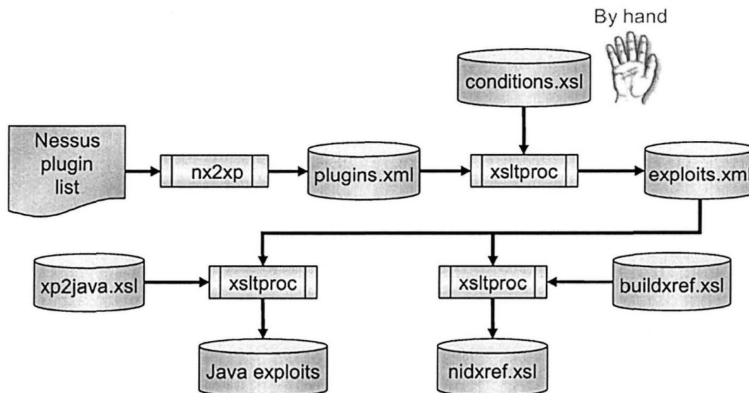
Figure 9-4. Generation of Exploits via Nessus
