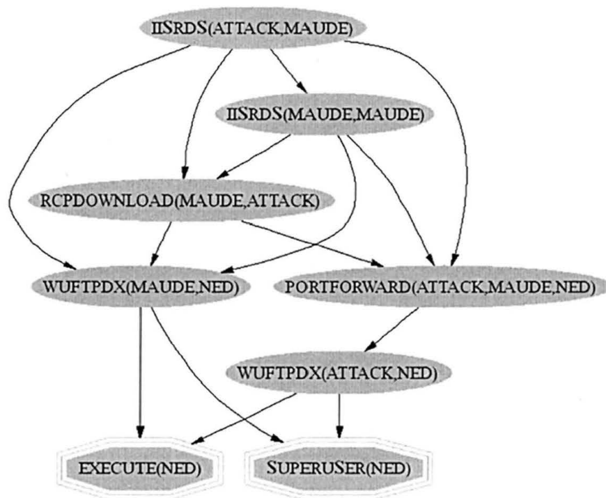
Figure 9-6. Attack Graph for Example Application of TVA
