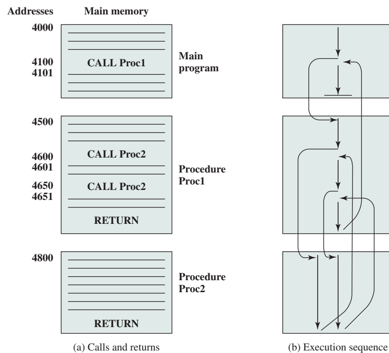
Figure 12.8 Nested Procedures
