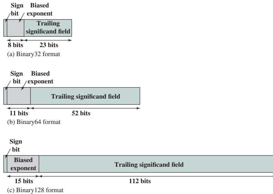
Figure 10.21 IEEE 754 Formats
