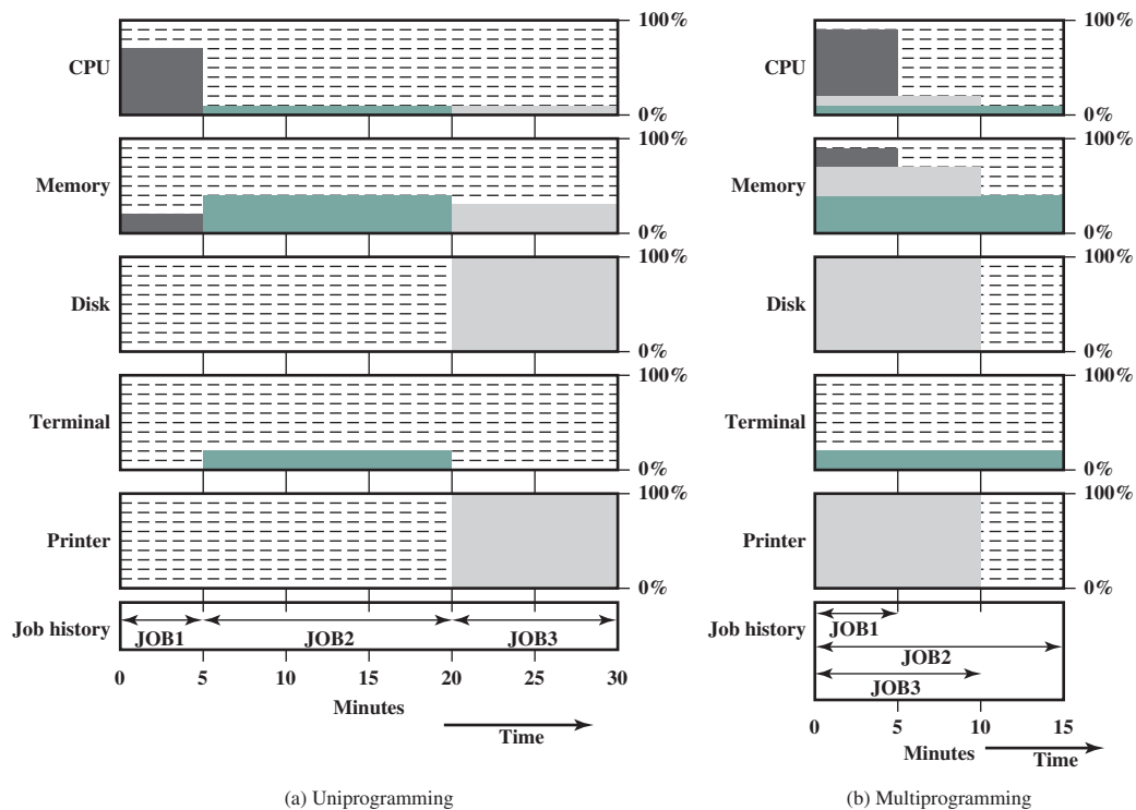
Figure 8.6 Utilization Histograms
