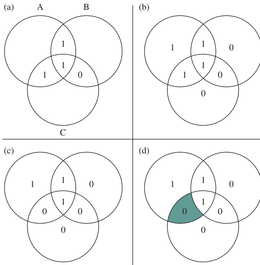
Figure 5.8 Hamming Error-Correcting Code
