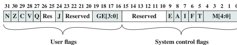
Figure 14.27 Format of ARM CPSR and SPSR
