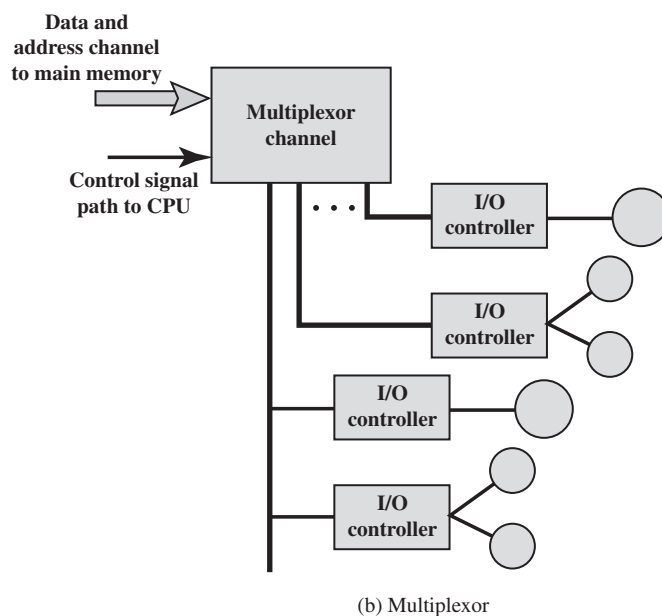
Figure 7.18 I/O Channel Architecture
