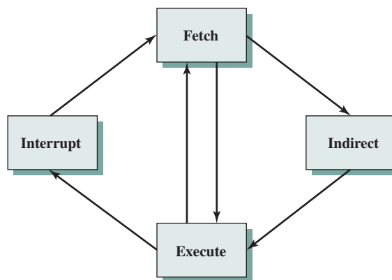
Figure 14.4 The Instruction Cycle
