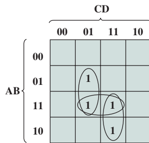
Figure 11.9 Overlapping Groups
