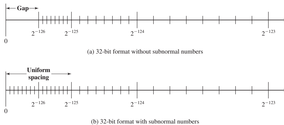
Figure 10.26 The Effect of IEEE 754 Subnormal Numbers
