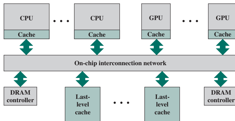
Figure 18.7 Heterogeneous Multicore Chip Elements
