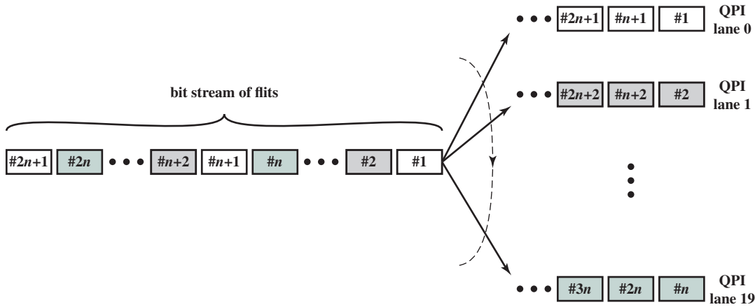
Figure 3.20 QPI Multilane Distribution
