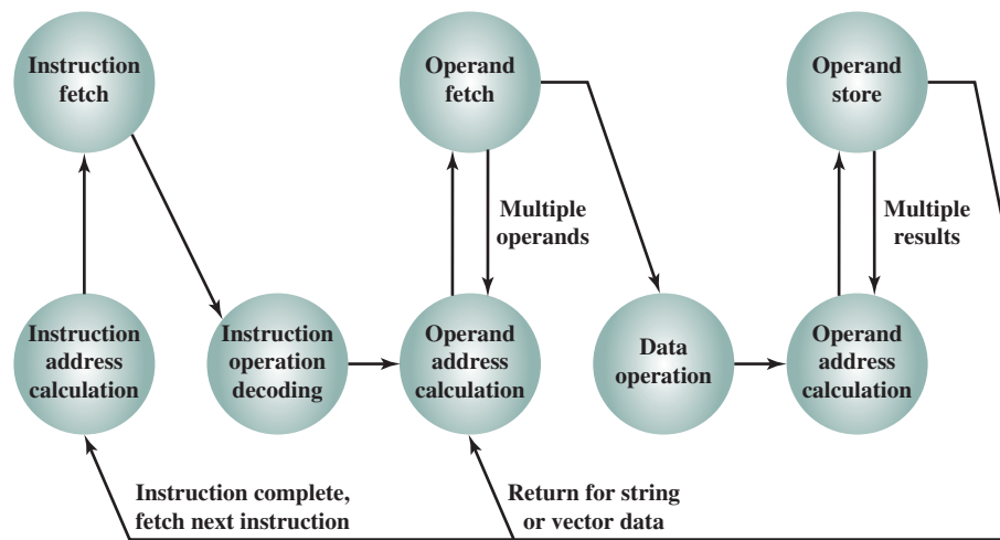
Figure 3.6 Instruction Cycle State Diagram
