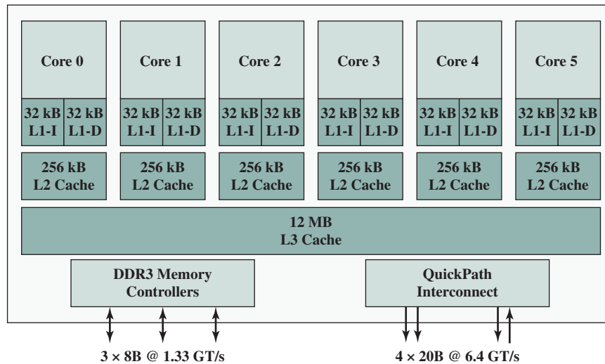
Figure 18.13 Intel Core i7-990X Block Diagram
