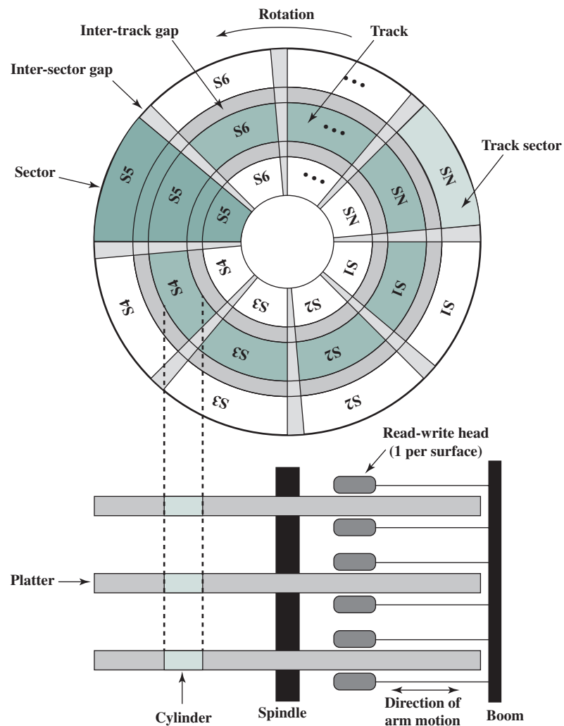
Figure 6.2 Disk Data Layout
