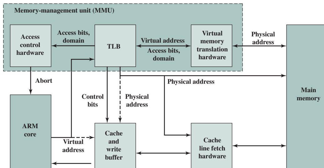
Figure 8.22 ARM Memory System Overview
