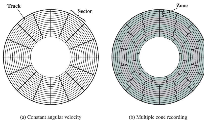
Figure 6.3 Comparison of Disk Layout Methods
