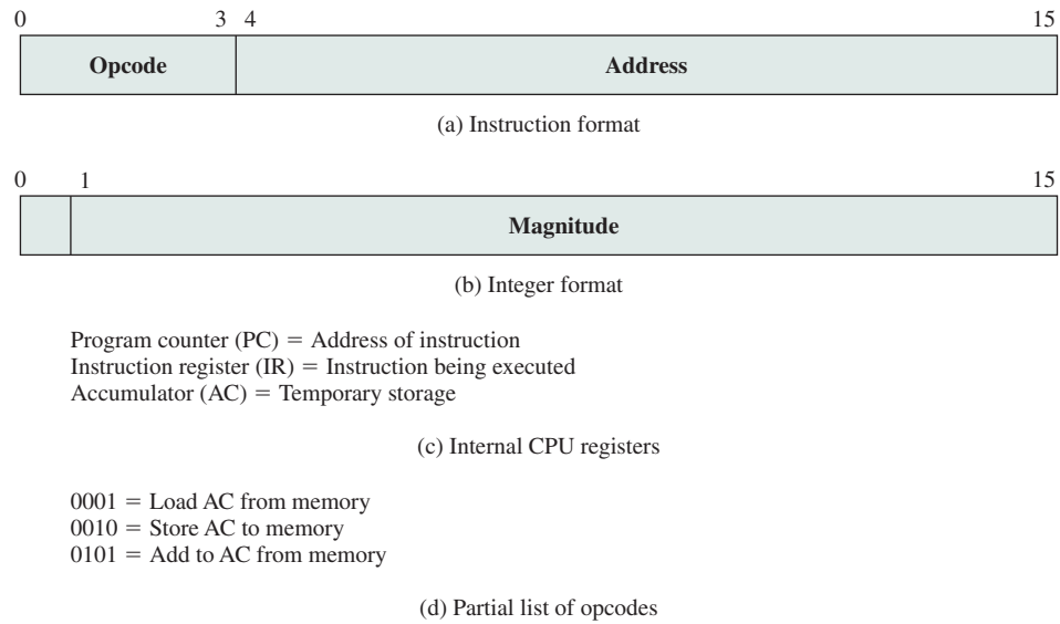
Figure 3.4 Characteristics of a Hypothetical Machine
