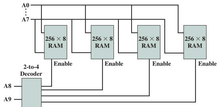
Figure 11.16 Address Decoding
