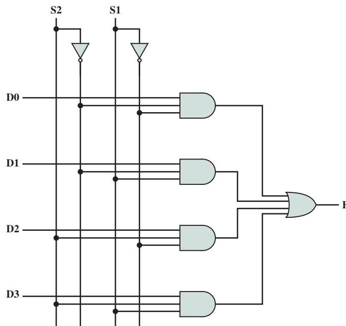
Figure 11.13 Multiplexer Implementation
