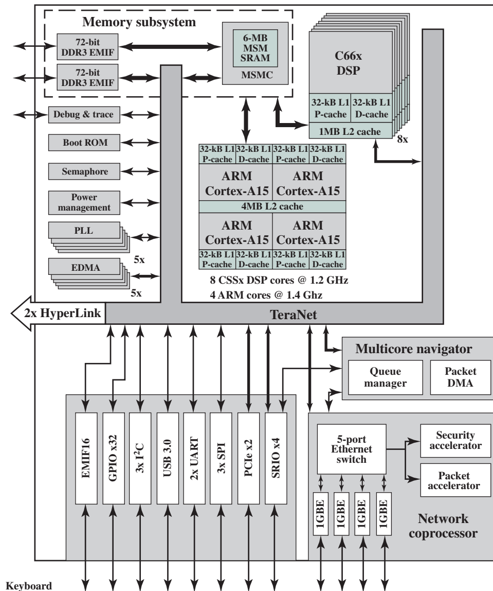
Figure 18.8 Texas Instruments 66AK2H12 Heterogeneous Multicore Chip
