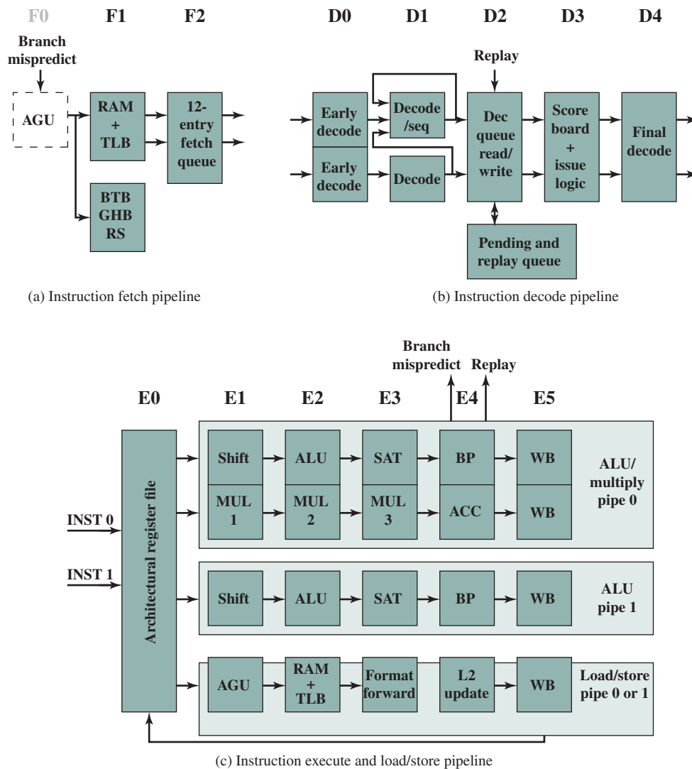
Figure 16.10 ARM Cortex-A8 Integer Pipeline
