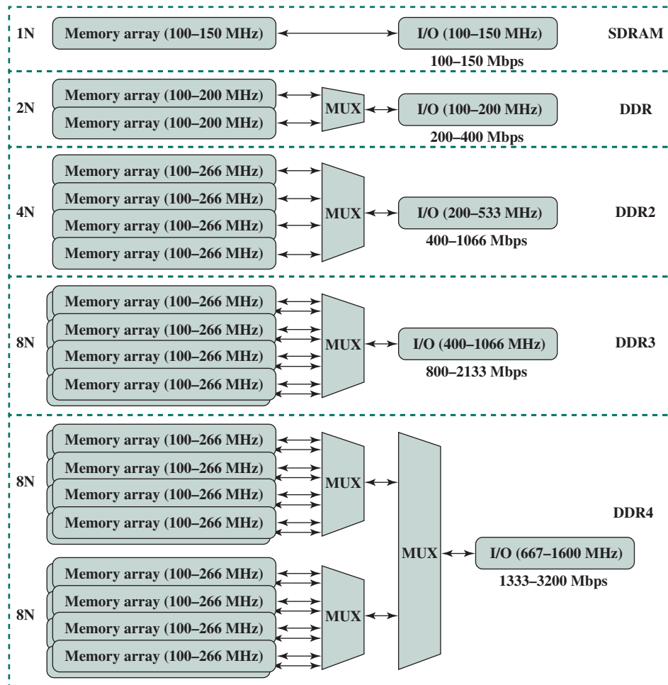
Figure 5.14 DDR Generations
