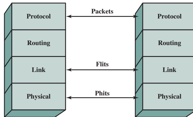
Figure 3.18 QPI Layers
