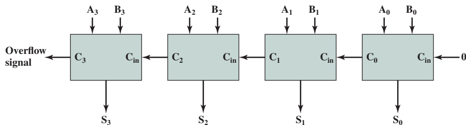
Figure 11.19 4-Bit Adder
