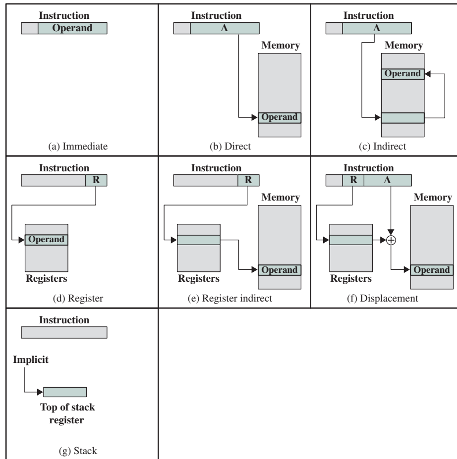
Figure 13.1 Addressing Modes
