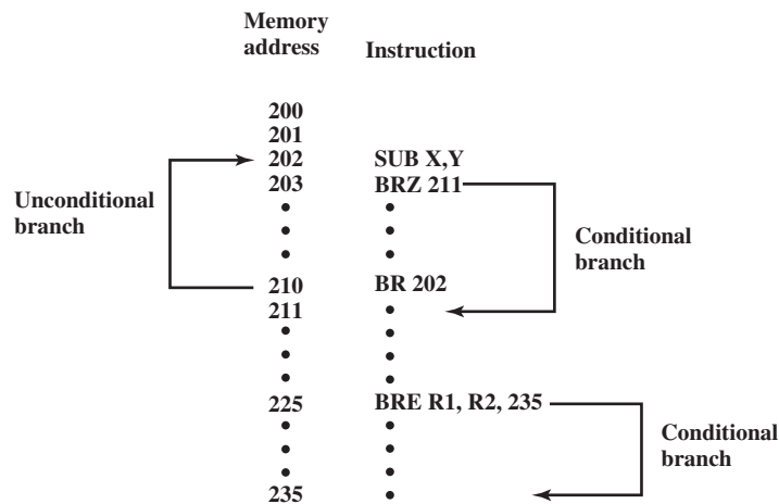
Figure 12.7 Branch Instructions
