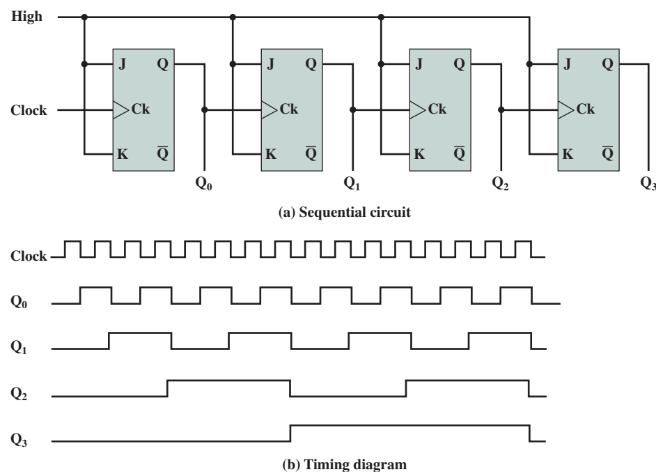
Figure 11.30 Ripple Counter
