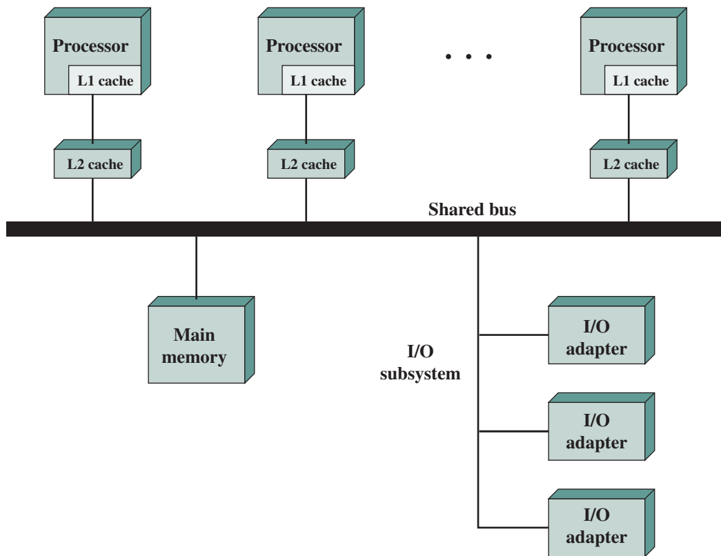
Figure 17.5 Symmetric Multiprocessor Organization
