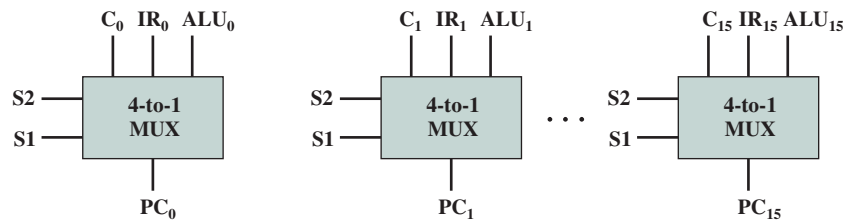
Figure 11.14 Multiplexer Input to Program Counter
