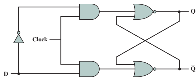
Figure 11.25 D Flip-Flop
