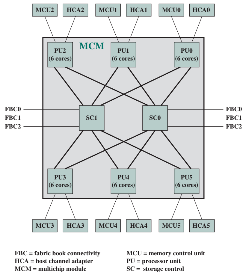
Figure 18.16 IBM EC12 Processor Node Structure
