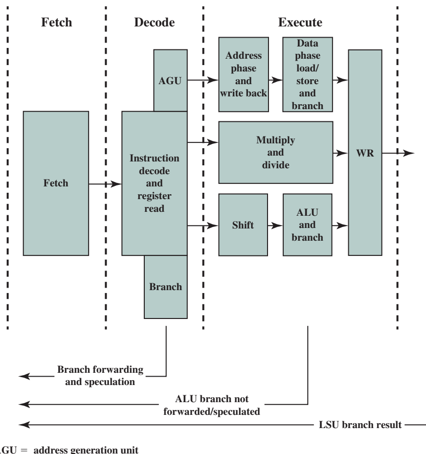
Figure 16.13 ARM Cortex-M3 Pipeline
