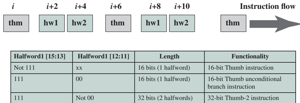
Figure 13.13 Thumb-2 Encoding
