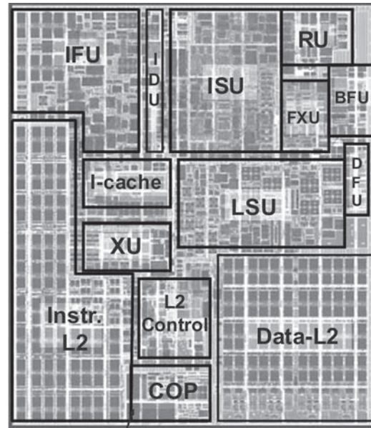
Figure 1.5 zEnterprise EC12 Core layout
