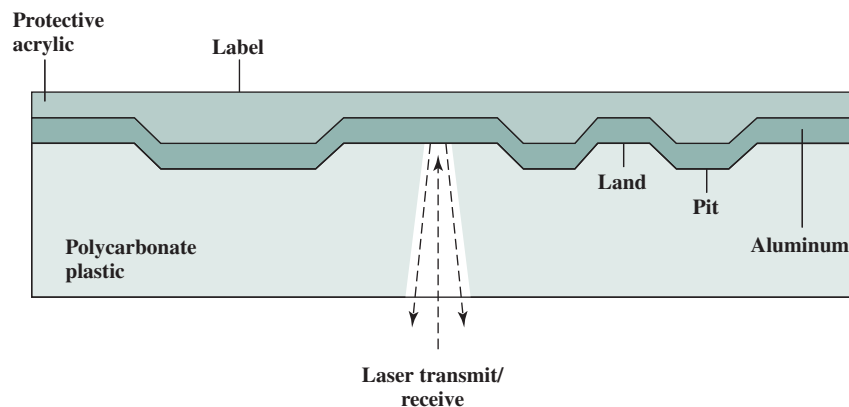
Figure 6.9 CD Operation
