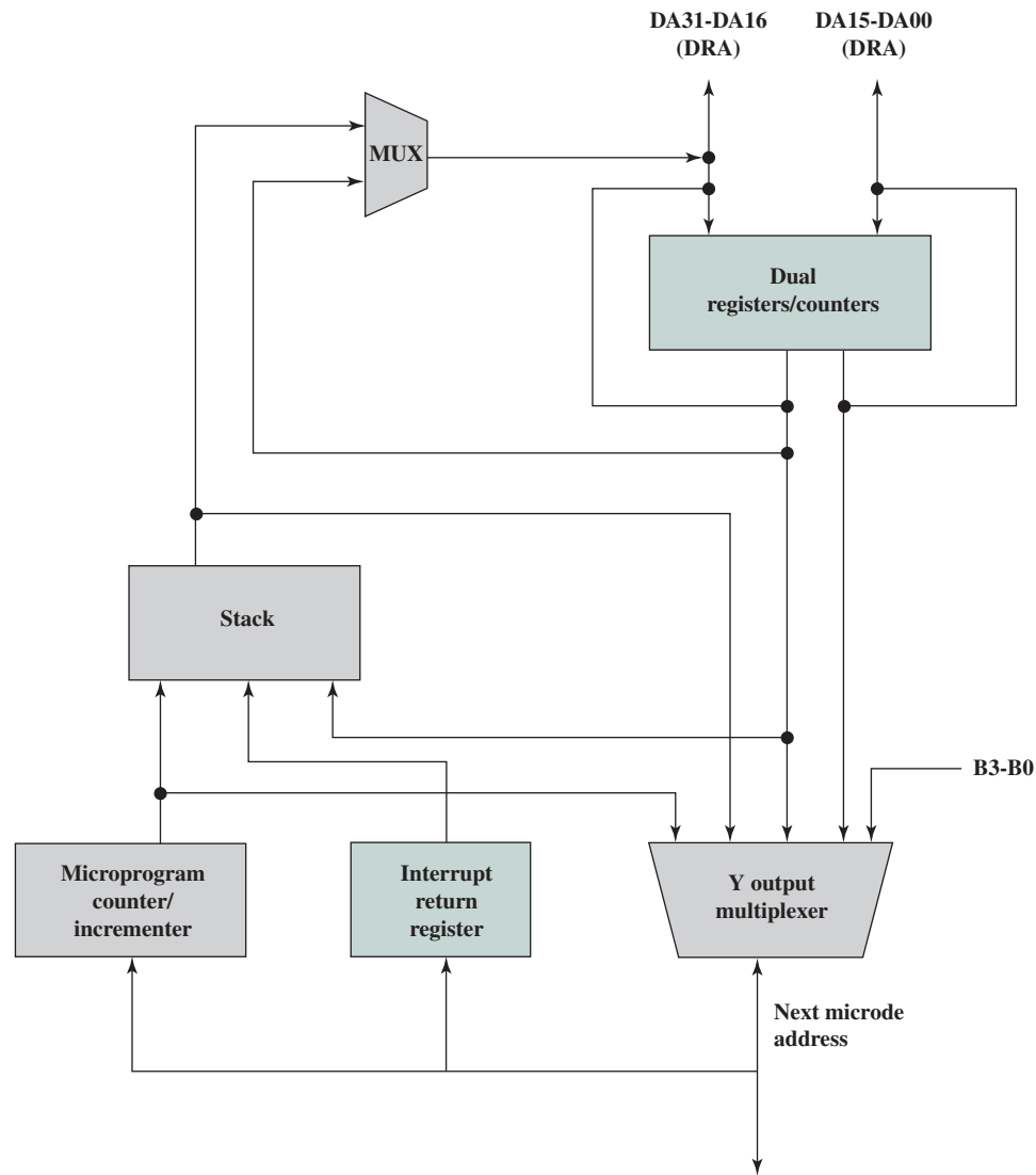
Figure 21.18 TI 8818 Microsequencer
