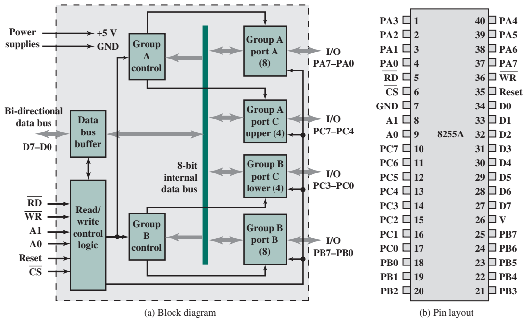
Figure 7.9 The Intel 8255A Programmable Peripheral Interface
