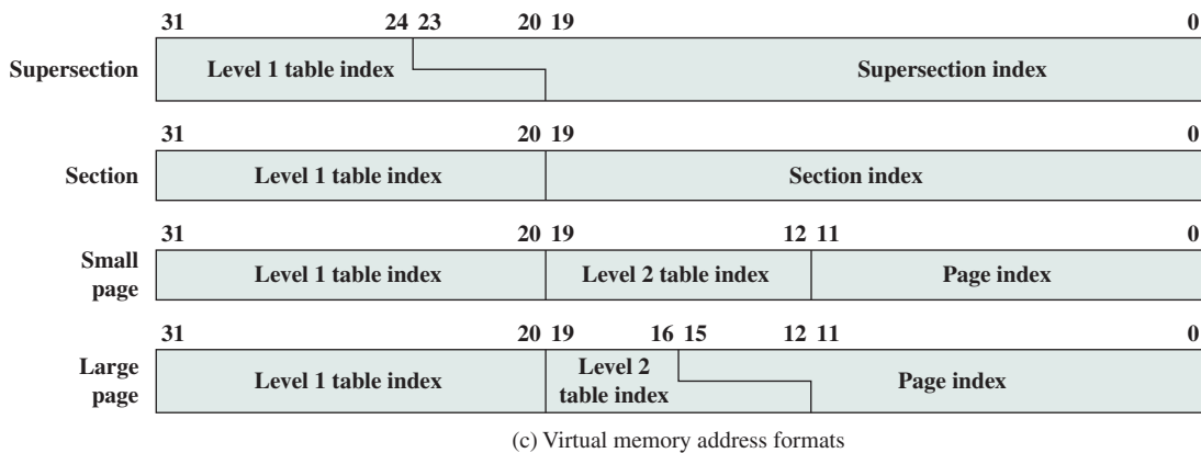
Figure 8.24 ARM Memory-Management Formats
