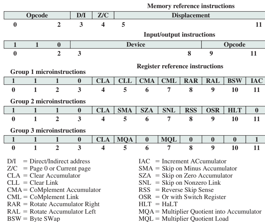
Figure 13.5 PDP-8 Instruction Formats
