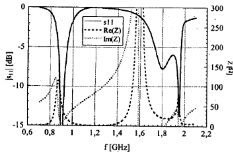
a) Matching and impedance behavior.
