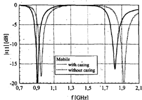
Figure 4: Matching of the dualband antenna with/without plastic casing.
