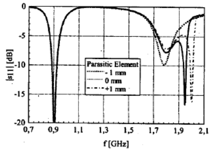
b) Variation of the parasitic element.
