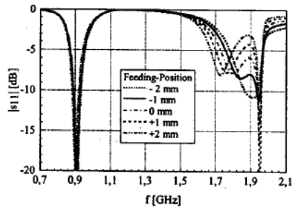
c) Variation of feeding point.
