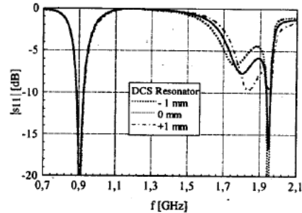
a) Variation of the DCS resonator.
