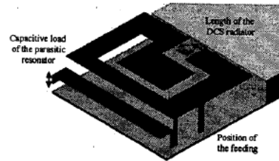
Figure 7: Parameters for tuning the coupling.
