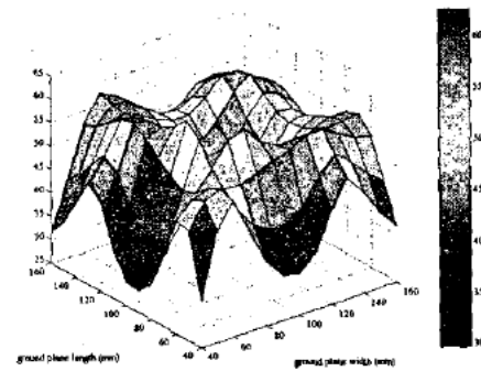
Figure 9: UMTS input resistances ( \Omega ).
