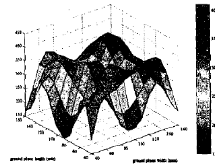
Figure 13: UMTS 80% antenna efficiency bandwidths (MHz).
