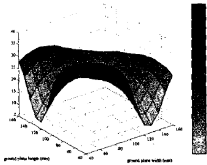
Figure 6: GSM900 unloaded quality factors.
