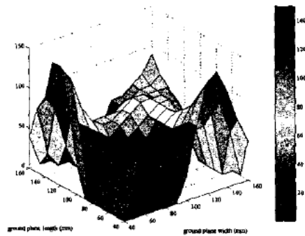
Figure 7: GSM900 80% antenna efficiency bandwidths (MHz).
