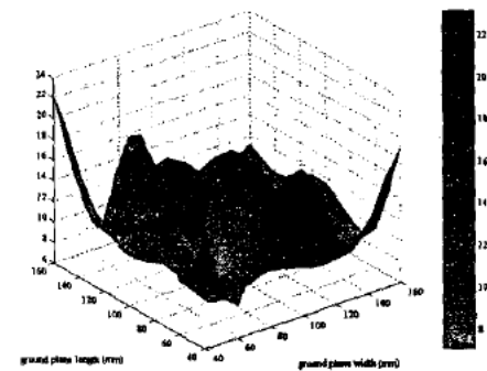
Figure 12: UMTS unloaded quality factors.
