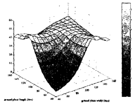
Figure 3: GSM900 input resistances ( \Omega ).
