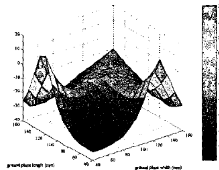
Figure 4: GSM900 input reactances ( \Omega ).
