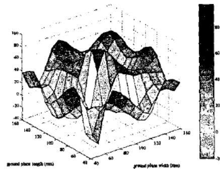
Figure 8: UMTS resonance frequencies (MHz from center frequency).
