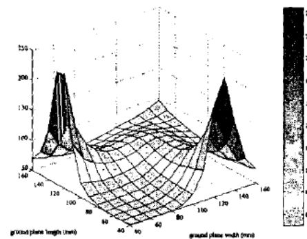
Figure 5: GSM900 6dB impedance bandwidths (MHz).
