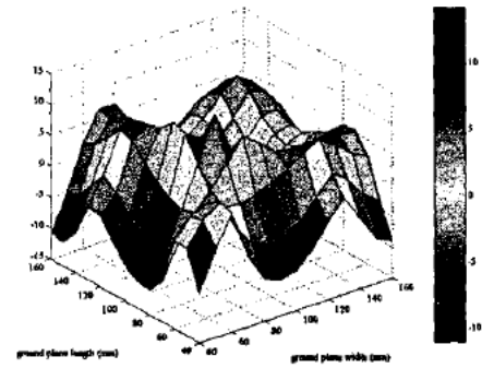
Figure 10: UMTS input reactances ( \Omega ).
