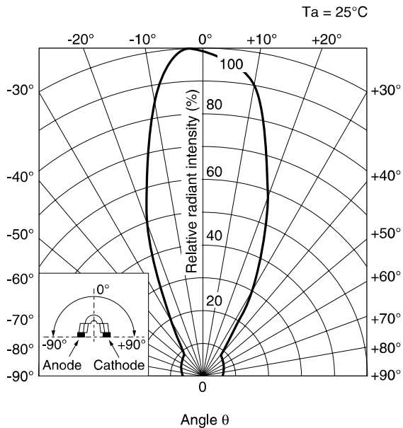
Fig. 3 Radiation Diagram (TYP.)
