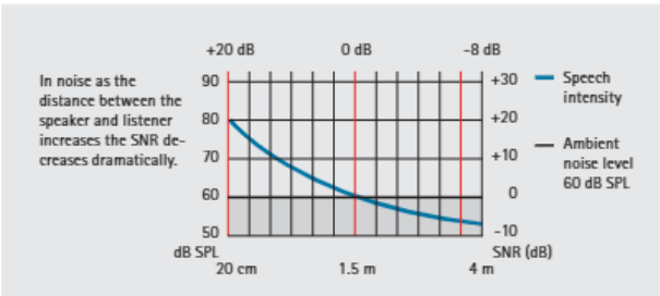
Speech-to-Noise Ratio without FM is distance dependent
