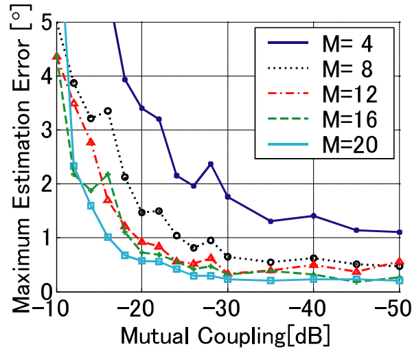
Fig.3: Maximum value of estimation error as a function of mutual coupling ( NA_{\text{std}}: 1\text{dB} , N\phi_{\text{std}}: 5^\circ ).
