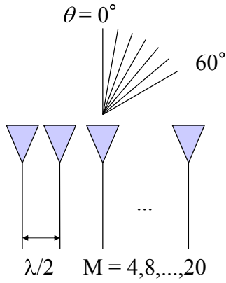
Fig. 1: Array antenna and direction.
