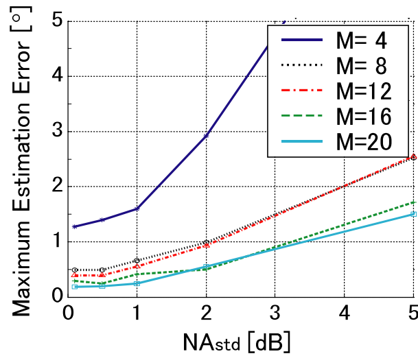
Fig.4: Maximum value of estimation error as a function of NA_{\text{std}} ( A_2: -30\text{dB} ).
