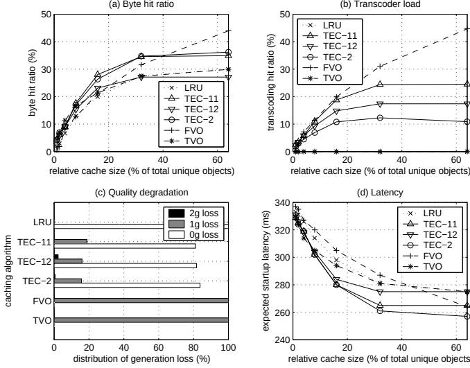
Fig. 5. Performance comparison in model-based simulations.
