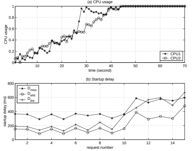
Fig. 10. CPU usage and delay.
