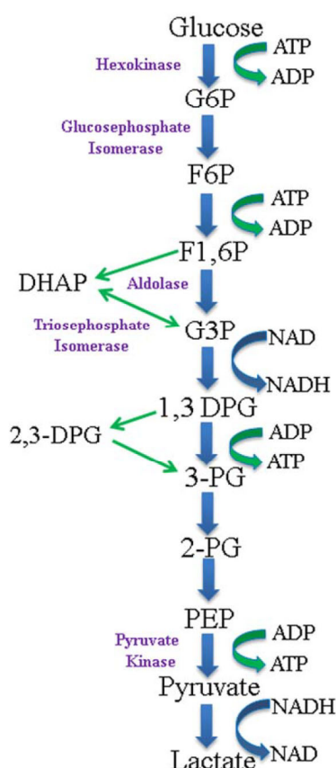
Figure 1. The Emden-Meyerhof pathway. G6P, glucose-6-phosphate; F6P, fructose-6-phosphate; F1,6P, fructose 1,6-phosphate; DHAP, dihydroxyacetone phosphate; G3P, glucose-3-phosphate; 1,3-DPG, 1,3-diphosphoglycerate; 2,3-DPG, 2,3-diphosphoglycerate; 3-PG, 3-phosphoglycerate; 2-PG, 2-phosphoglycerate; PEP, phosphoenolpyruvate. [Color figure can be viewed in the online issue, which is available at wileyonlinelibrary.com .]
