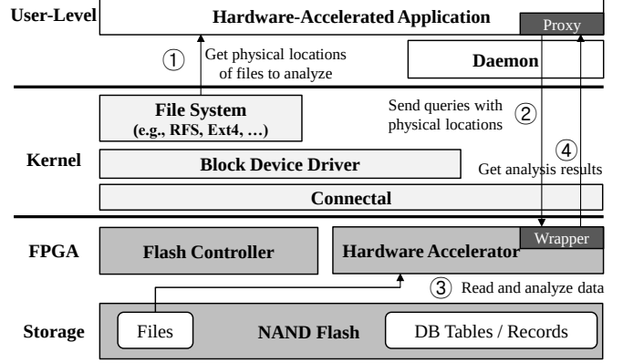
Figure 8: Software interface
