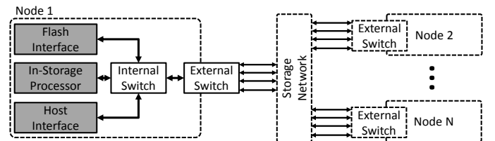
Figure 4: Network architecture
