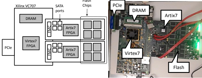
Figure 10: A BlueDBM storage node
