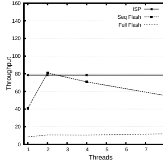
Figure 18: Nearest neighbor with off-the-shelf SSD
