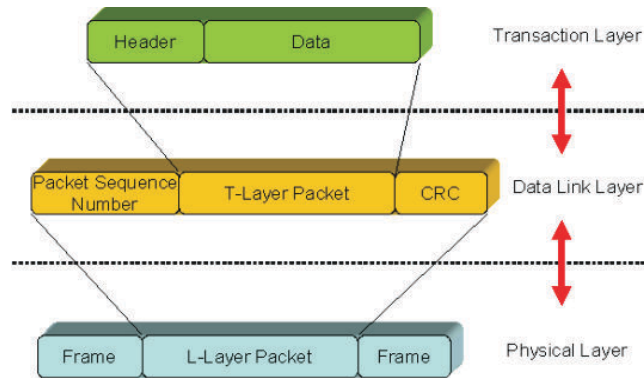
Figure 4: The data link layer adds data integrity features [1] .
