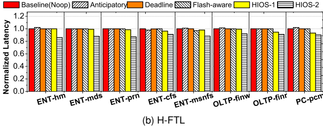
Figure 12: Average latencies for two different types of FTLs (normalized to the noop scheduler).
