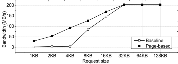
(b) Impact of page-based aggregation
