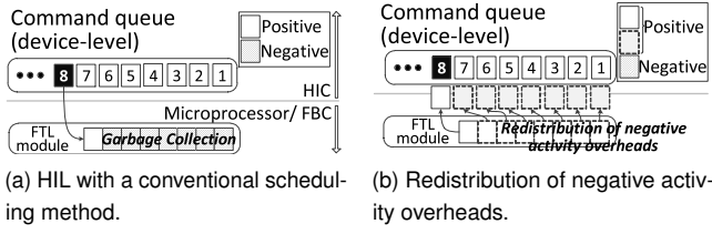
Figure 8: Comparison between HIL with a conventional scheduler and our proposed HIOS.
