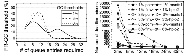
(a) Sensitivity to the number of queue entries and GC threshold. (b) Sensitivity to deadline period and GC threshold.
