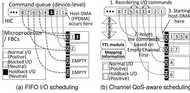
Figure 9: Illustration of performance degradation due to channel resource conflicts. While existing schedulers cannot serve recently-arrived requests 4 to 8, HIOS can immediately serve them by converting neutral activities into positive ones.
