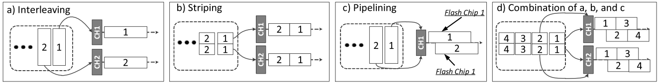
Figure 4: Three major types of parallelism within an SSD. Since each Flash Bus Controller (FBC) handles a channel, these different types of parallelism lead, in principle, to high-performance. However, if a channel is already allocated to other requests, issuing further requests to it generates a serialized access pattern that can result in performance degradation.
