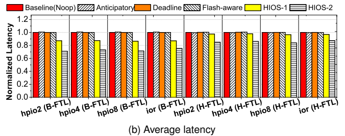
Figure 13: Latency comparison under the HPC workloads.
