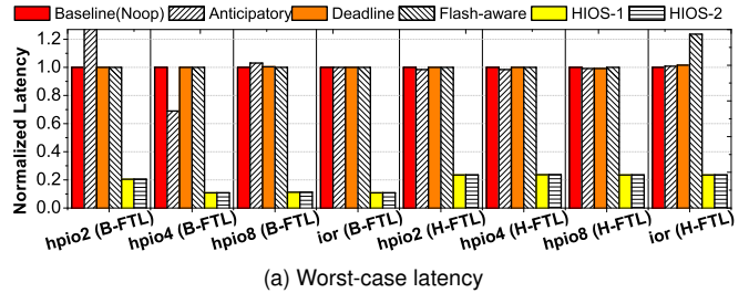
(a) Worst-case latency
