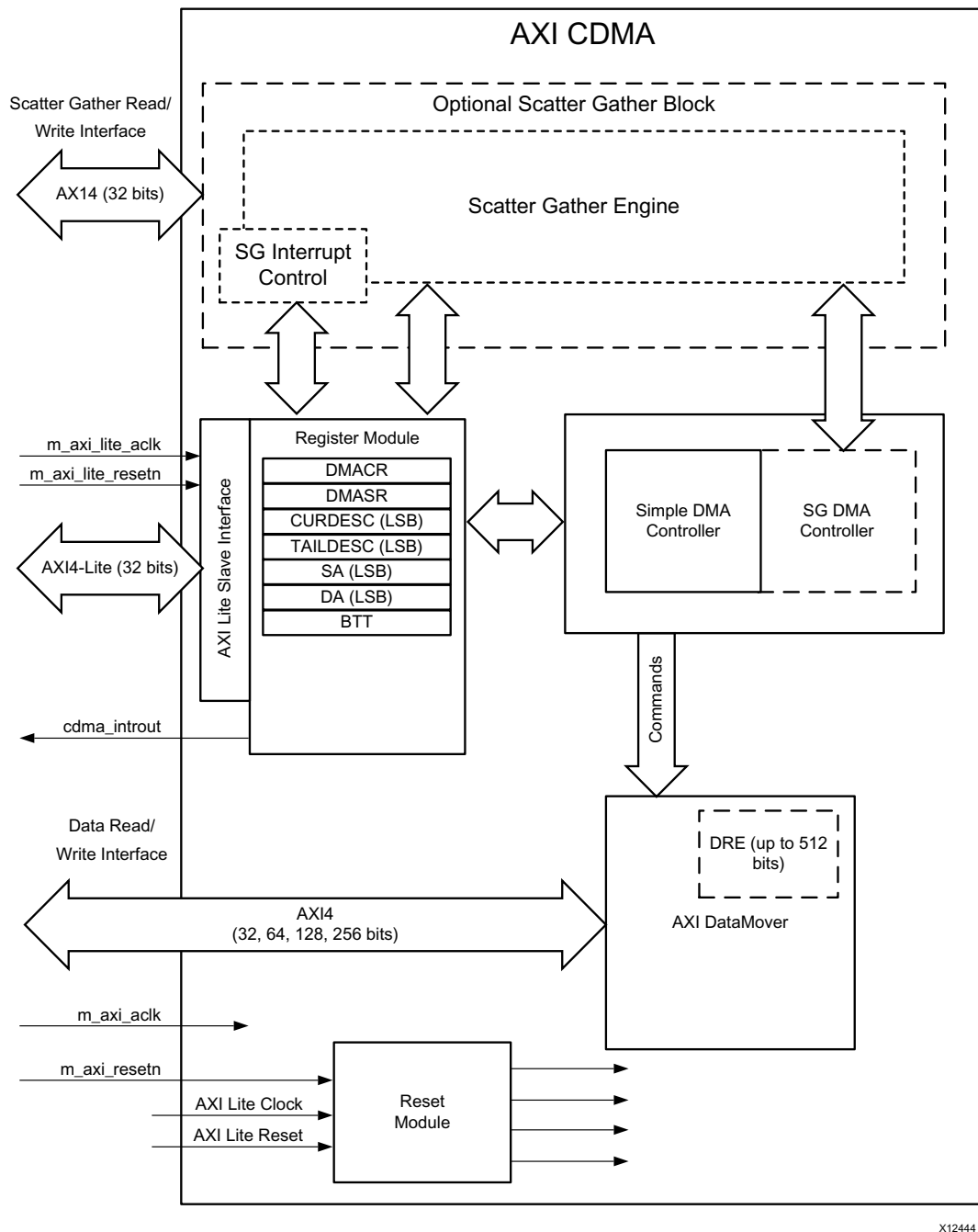
Figure 1-1: AXI CDMA Block Diagram
