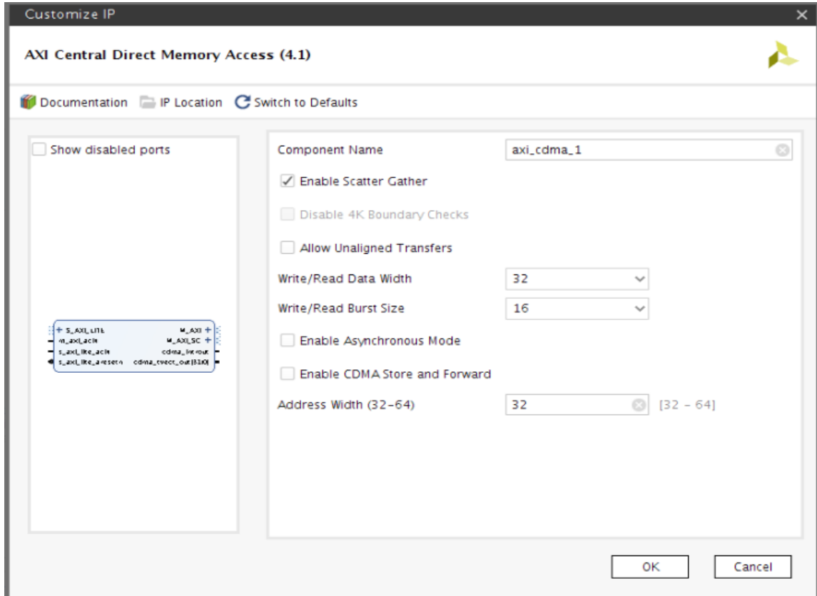
Figure 4-1: AXI CDMA Vivado IDE
