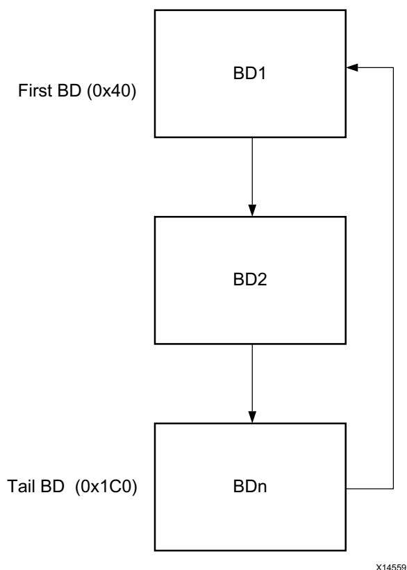
Figure 3-1: BD Chain
