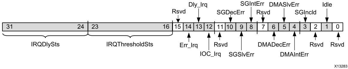
Figure 2-3: CDMASR Register
