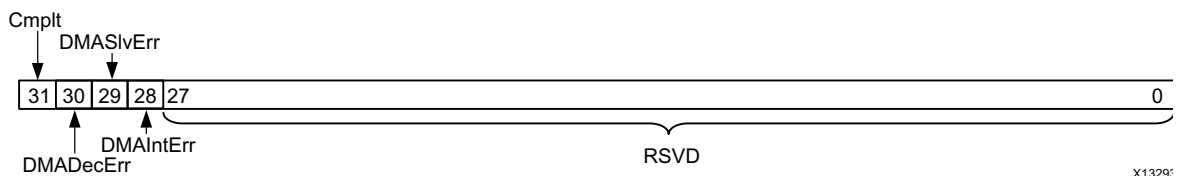
Figure 3-9: Transfer Descriptor Status Word
