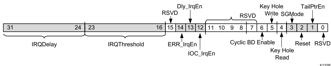
Figure 2-2: CDMACR Register
