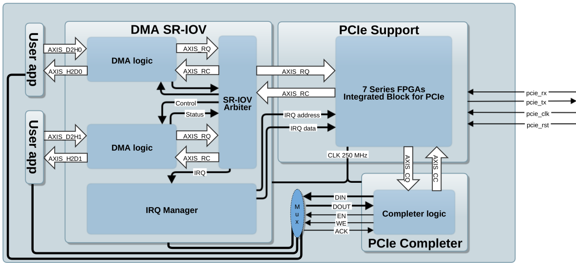
Fig. 3: Block diagram of the PCIe DMA engine
