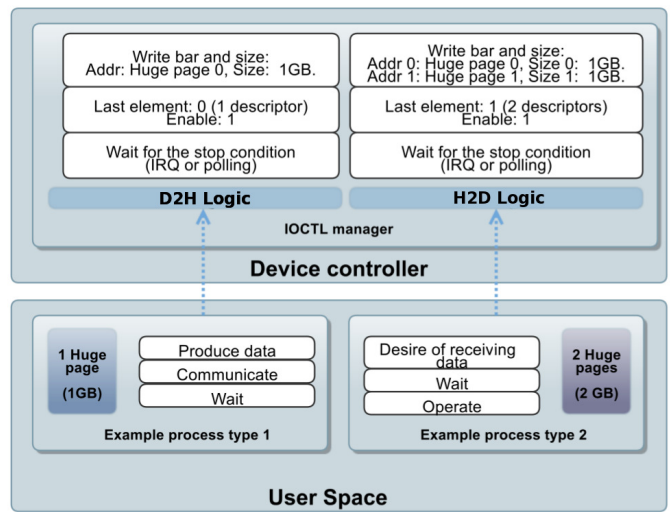
Fig. 5: Interfacing of the DMA core from User Space
