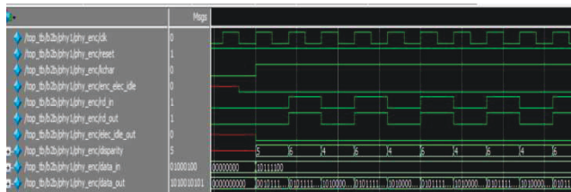
Fig -7: Input/output PHY 1 Encoder
