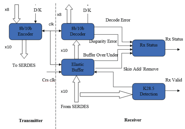
Fig -3: PCS Block Diagram
