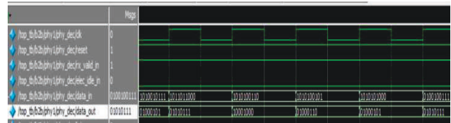
Fig -9: Input/output of PHY 1 Decoder
