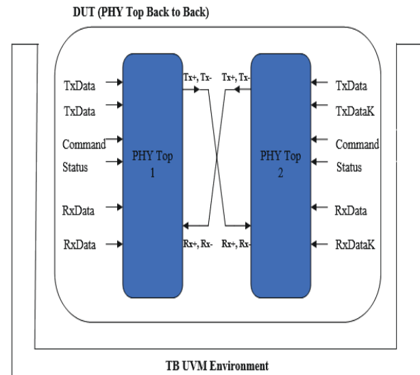
Fig -5: UVM Verification Environment for PHY (Loopback)
