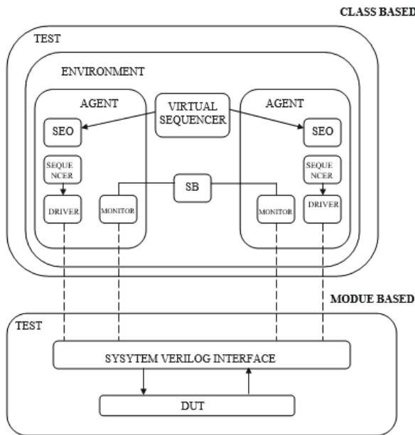
Fig -6: UVM Block Level Architecture and Test-Bench
