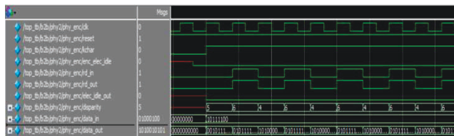
Fig -8: Input/output of PHY 2 Encoder
