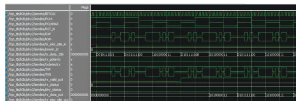
Fig -12: Input/output of PHY 2 SERDES
