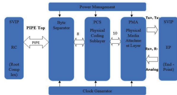
Fig -2: Partitioned physical layer for PCIe
