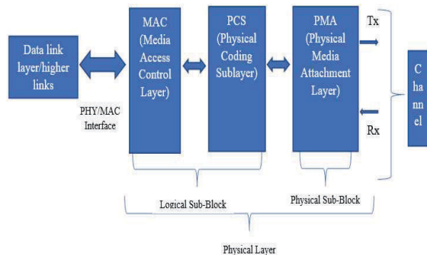
Fig -1: Partitioned physical layer for PCIe
