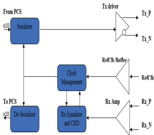
Fig -4: PMA Block Diagram
