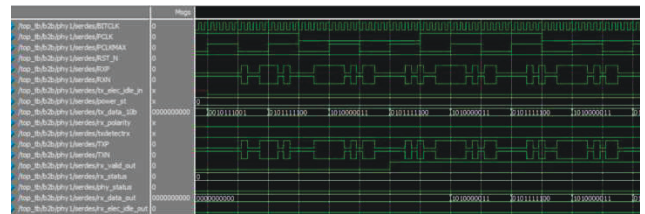
Fig -11: Input/output of PHY 1 SERDES
