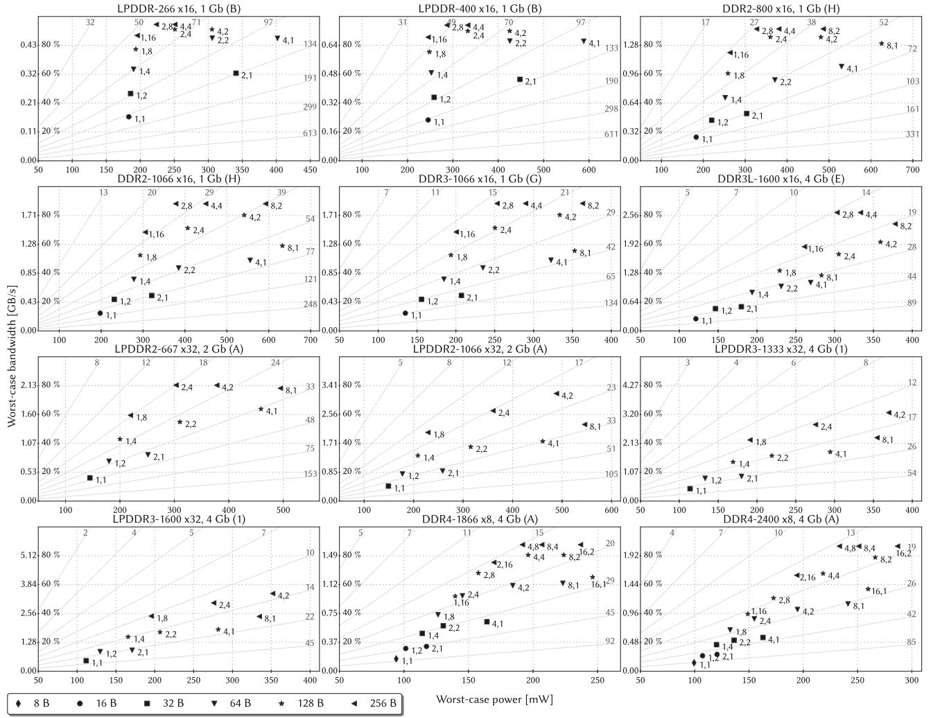
Fig. 8. Worst-case bandwidth versus worst-case power. The diagonal isolines connect points of equal energy efficiency, labeled with [pJ/bit] (125 divided by these labels yields [GB/J]). Percent-labels relate to the peak bandwidth.
