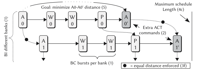
Fig. 6. ILP precedence constraints. An edge between two commands means that the source command must be scheduled before the destination command. Round brackets refer to rules in the ILP description.
