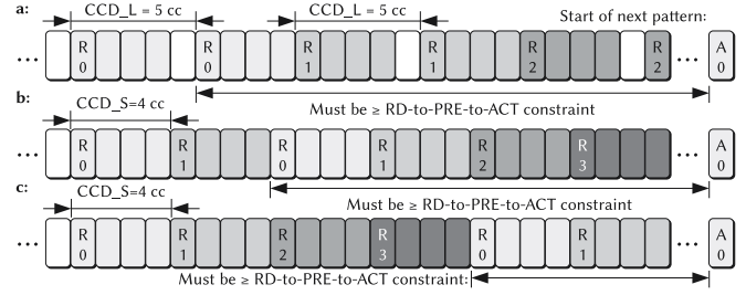
Fig. 3. (Partial) DDR4-1866 read pattern. Odd and even banks are in a different bank group. Schedule a does not use BS PBGI, while b does. c shows how the distance to the next activate in a following pattern reduces as more bank groups are interleaved, resulting in longer (less efficient) patterns.
