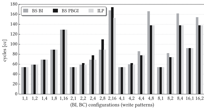
Fig. 7. Comparison of write pattern lengths for DDR4-1866, using bank scheduling (BS BI), bank scheduling with pairwise bank-group interleaving (BS PBGI) and the ILP formulation (ILP). Lower is better.
