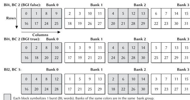
Fig. 5. Three memory map examples, showing where the bursts of requests to consecutive physical addresses (separated by the access granularity) are written. The third configuration, using (2, 1) behaves the same regardless of the BGI setting.
