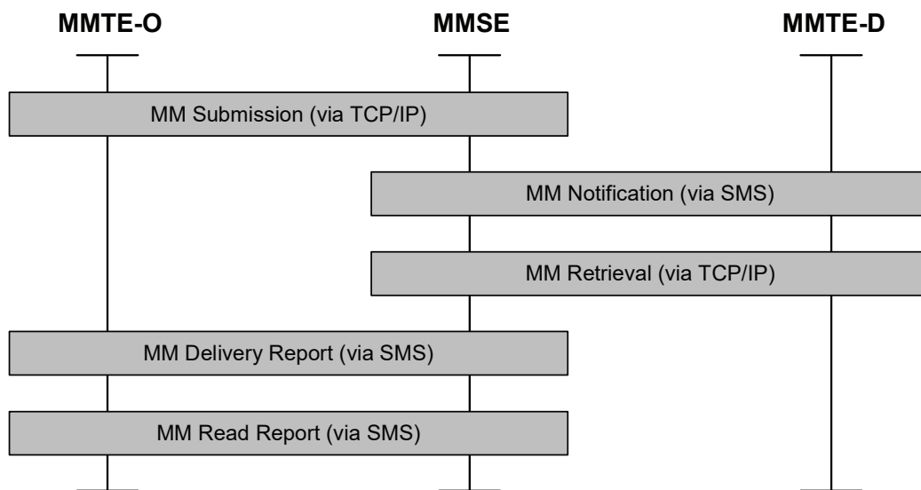
Figure 4: Generalized MMS transaction sequence in fixed networks
