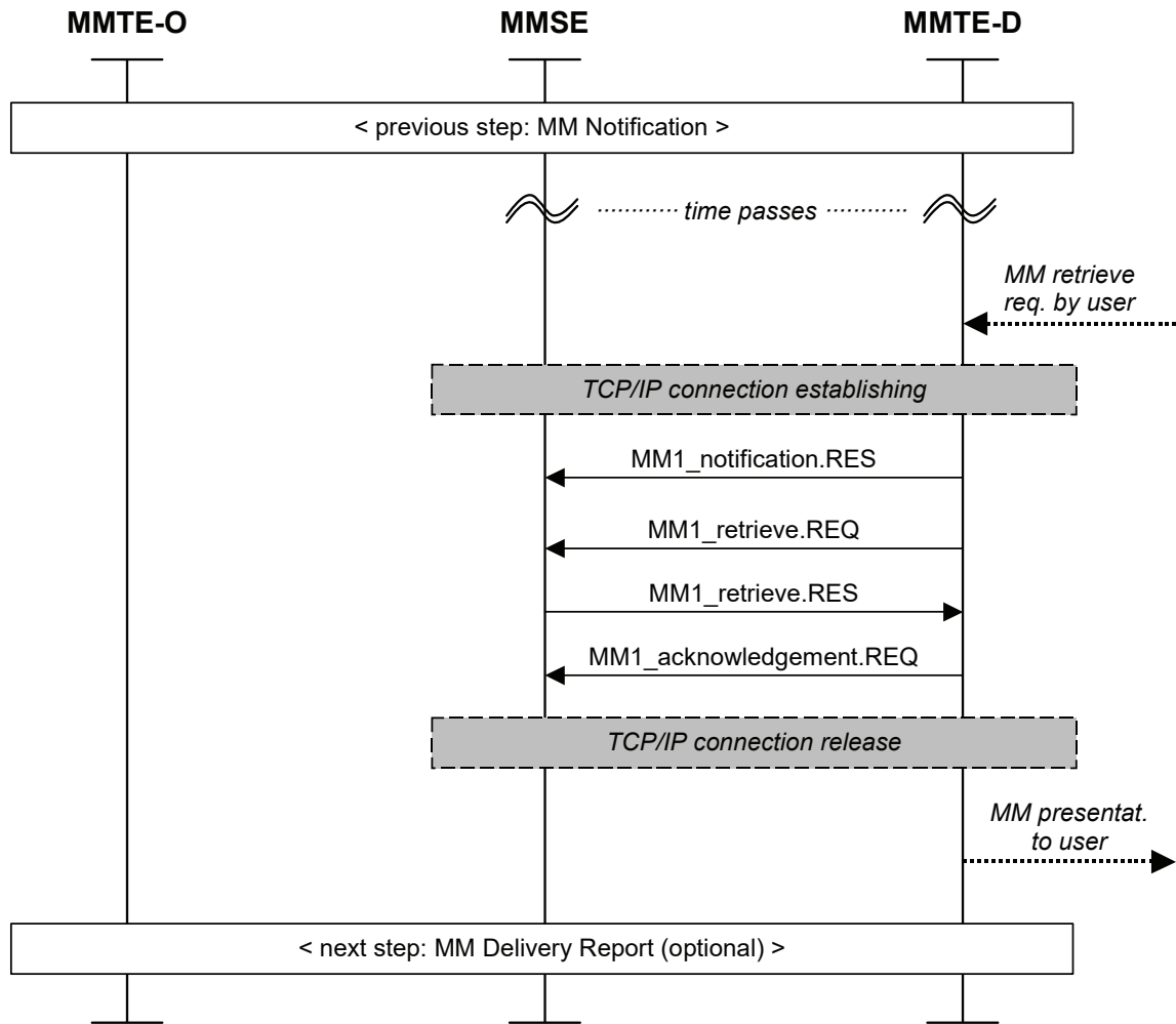
Figure 7: Example abstract message flow for MM Retrieval
