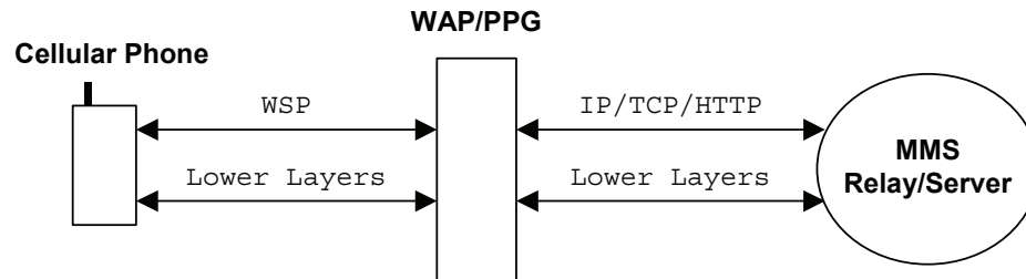
Figure 11: MM1 gateway structure in mobile networks
