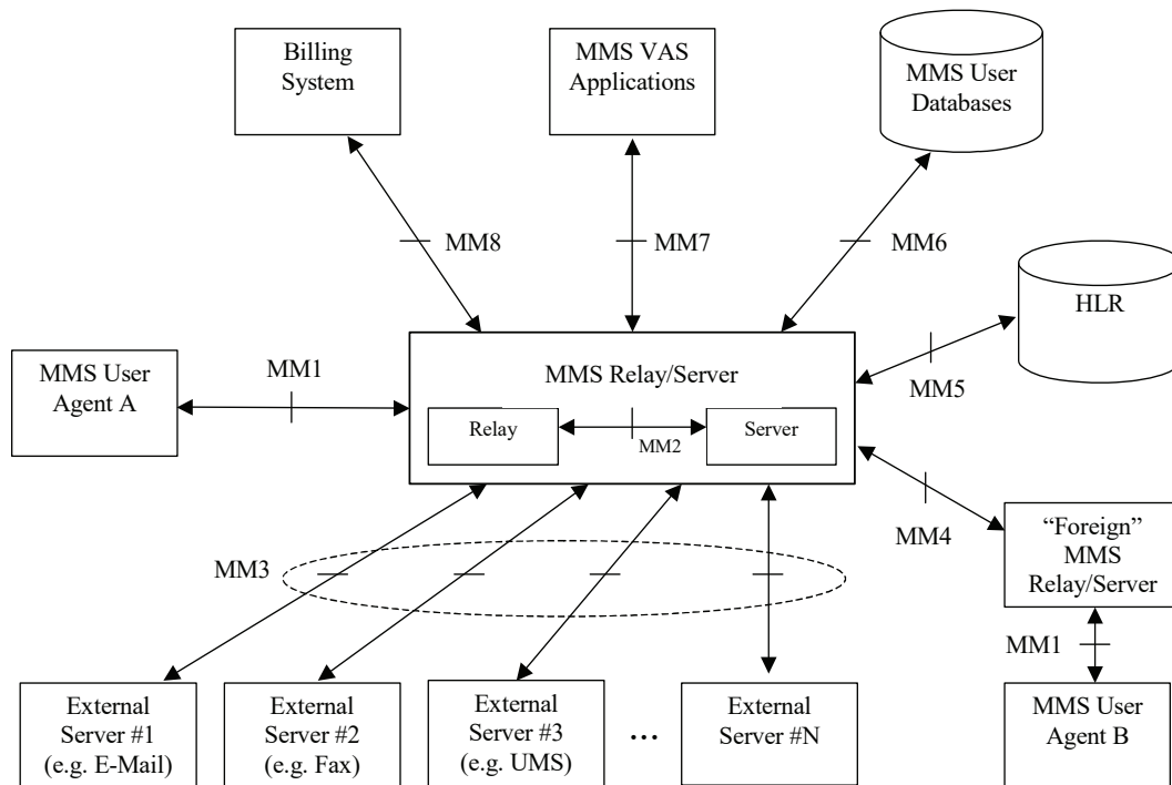
Figure 1: MMS Reference Architecture
