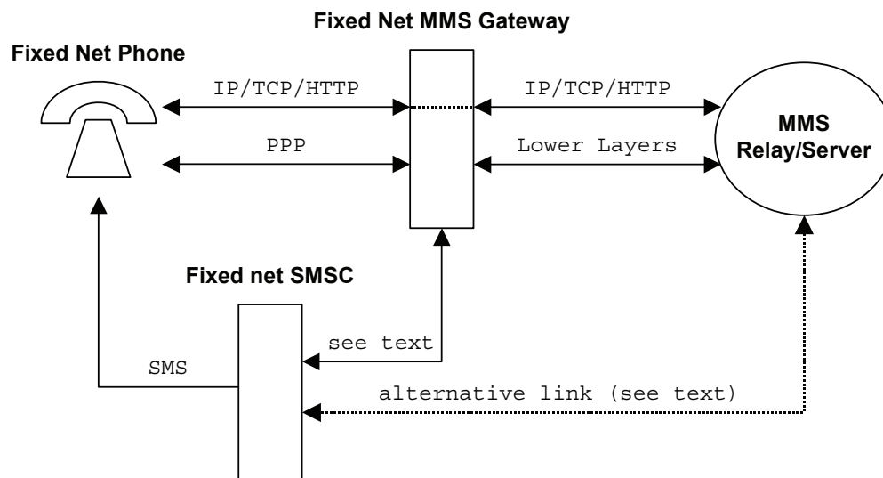
Figure 3: MM1 gateway structure for fixed networks
