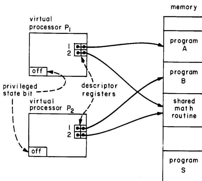
Fig. 3. Fig. 2 redrawn to show sharing of a math routine by two virtual processors simultaneously.
